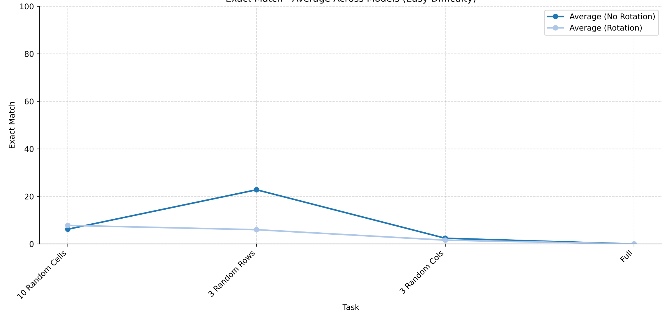
Exact Match - Average Across Models (Easy Difficulty)
