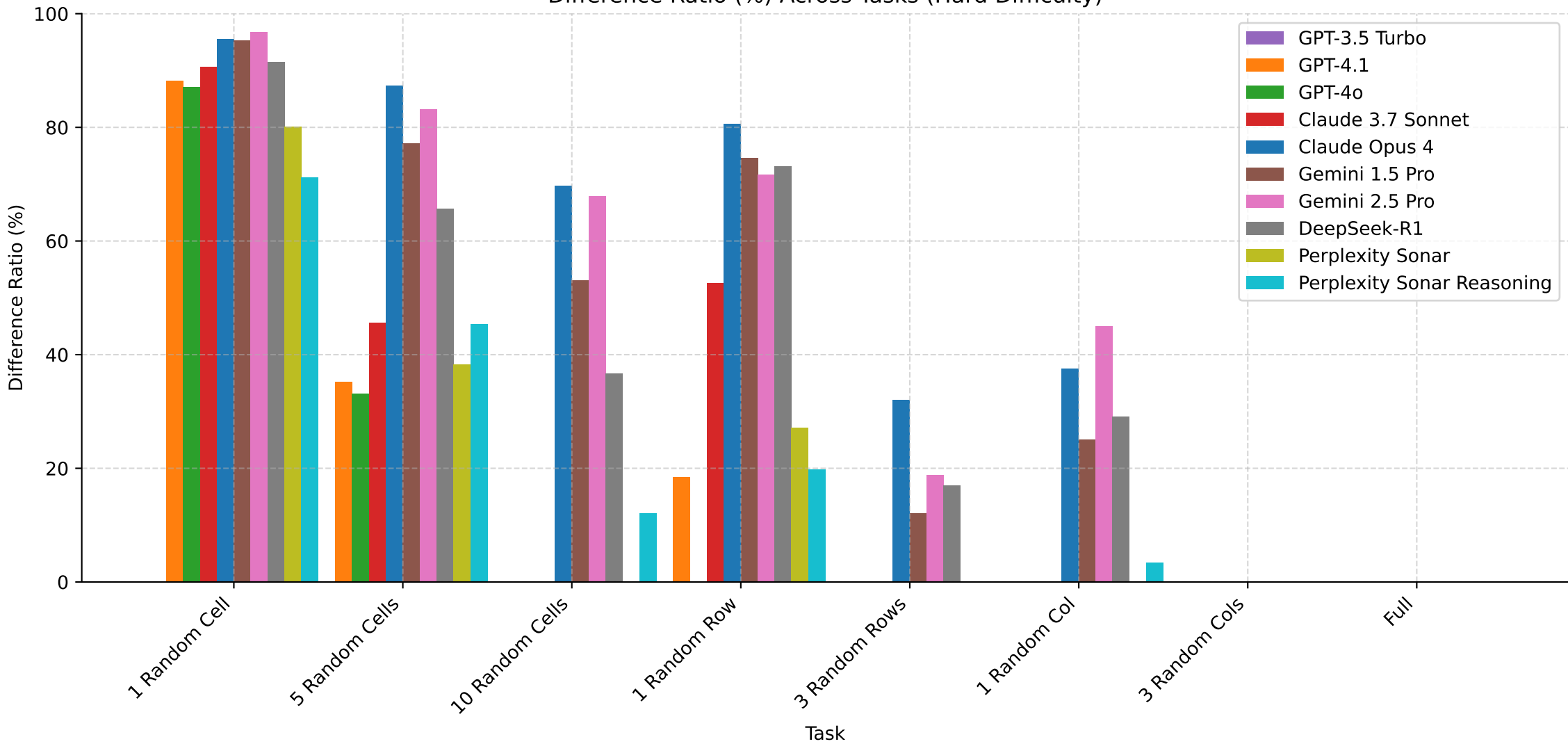
Difference Ratio (%) Across Tasks (Hard Difficulty)
