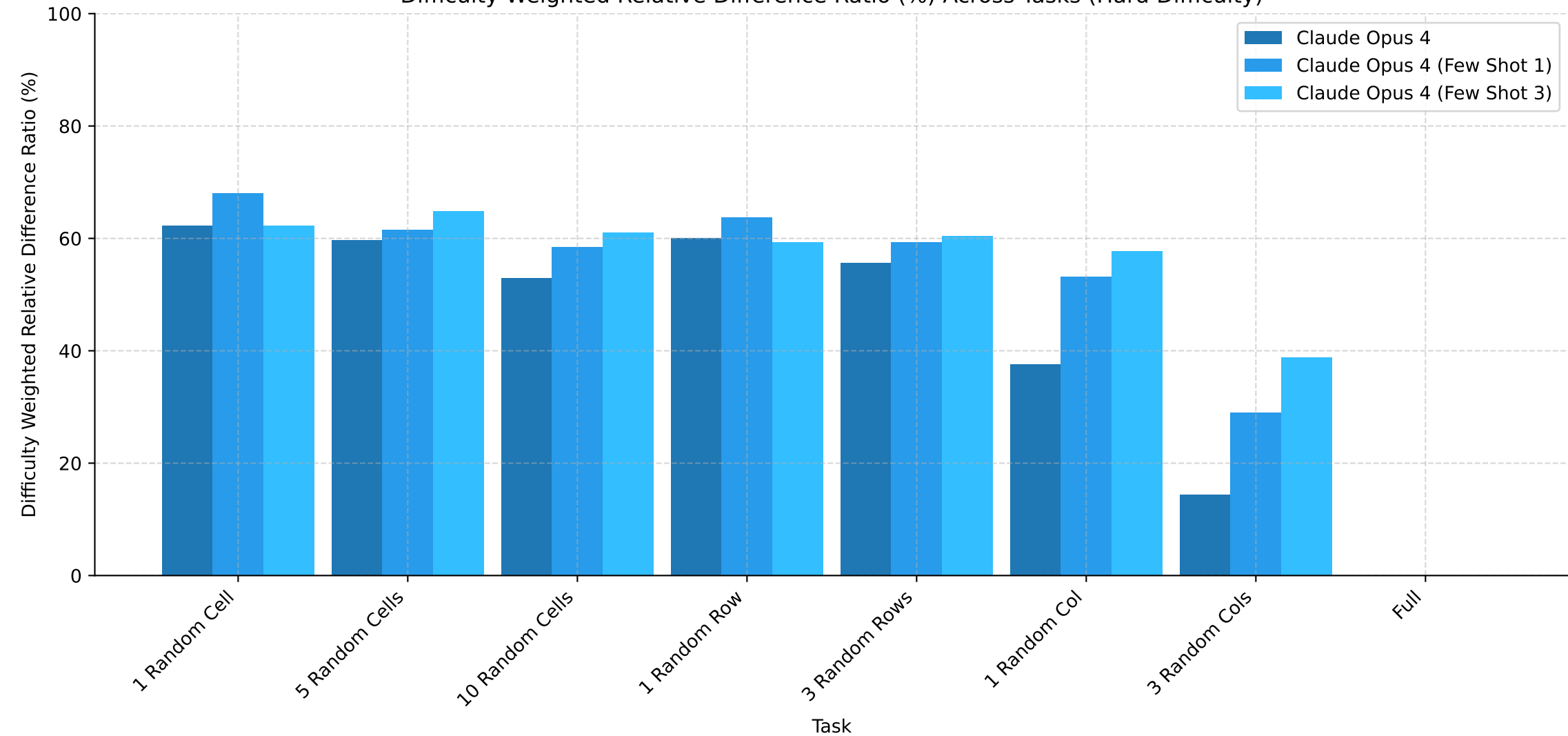
Difficulty Weighted Relative Difference Ratio (%) Across Tasks (Hard Difficulty)
