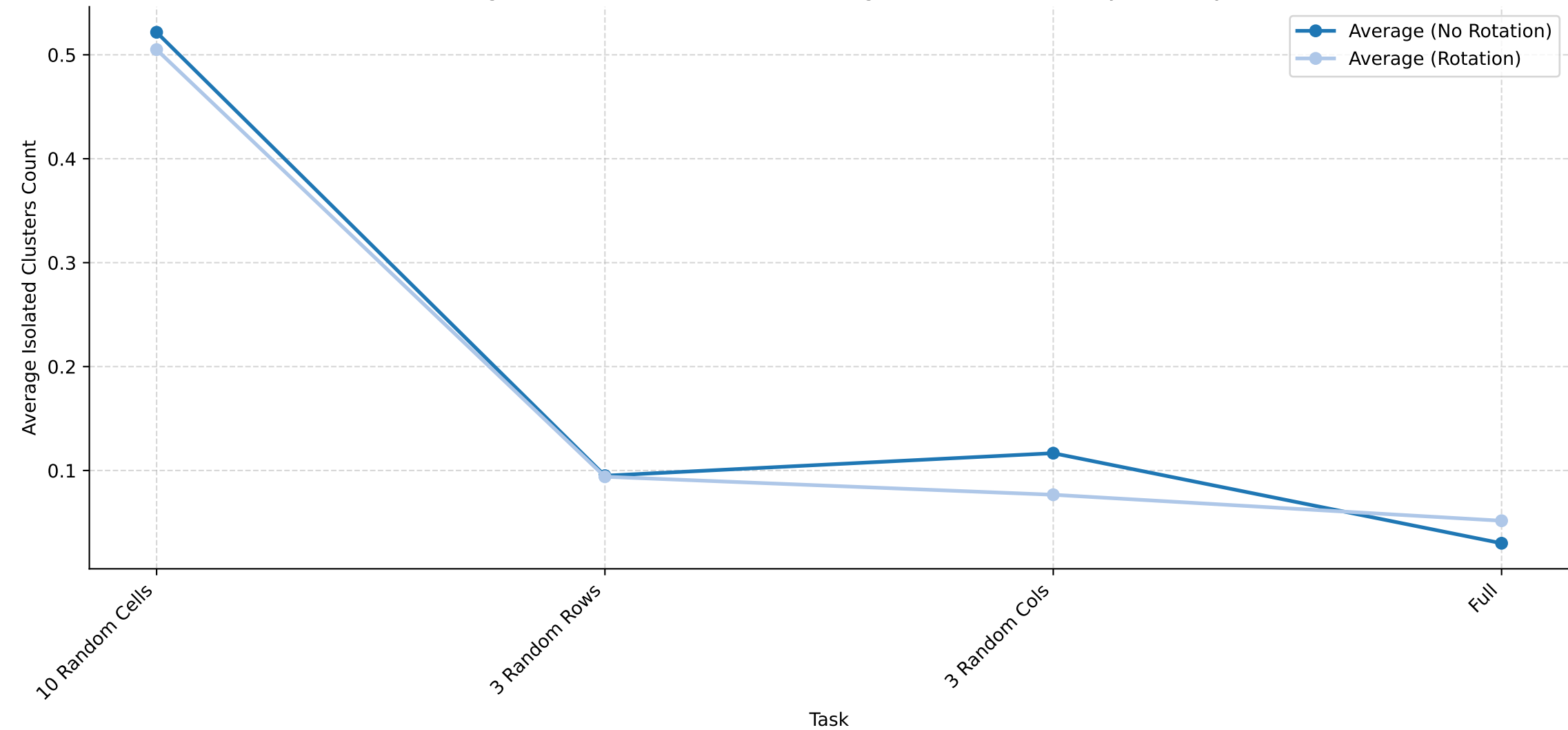
Average Isolated Clusters Count - Average Across Models (Easy Difficulty)
