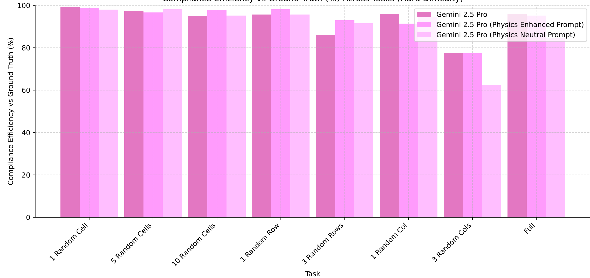
Compliance Efficiency vs Ground Truth (%) Across Tasks (Hard Difficulty)
