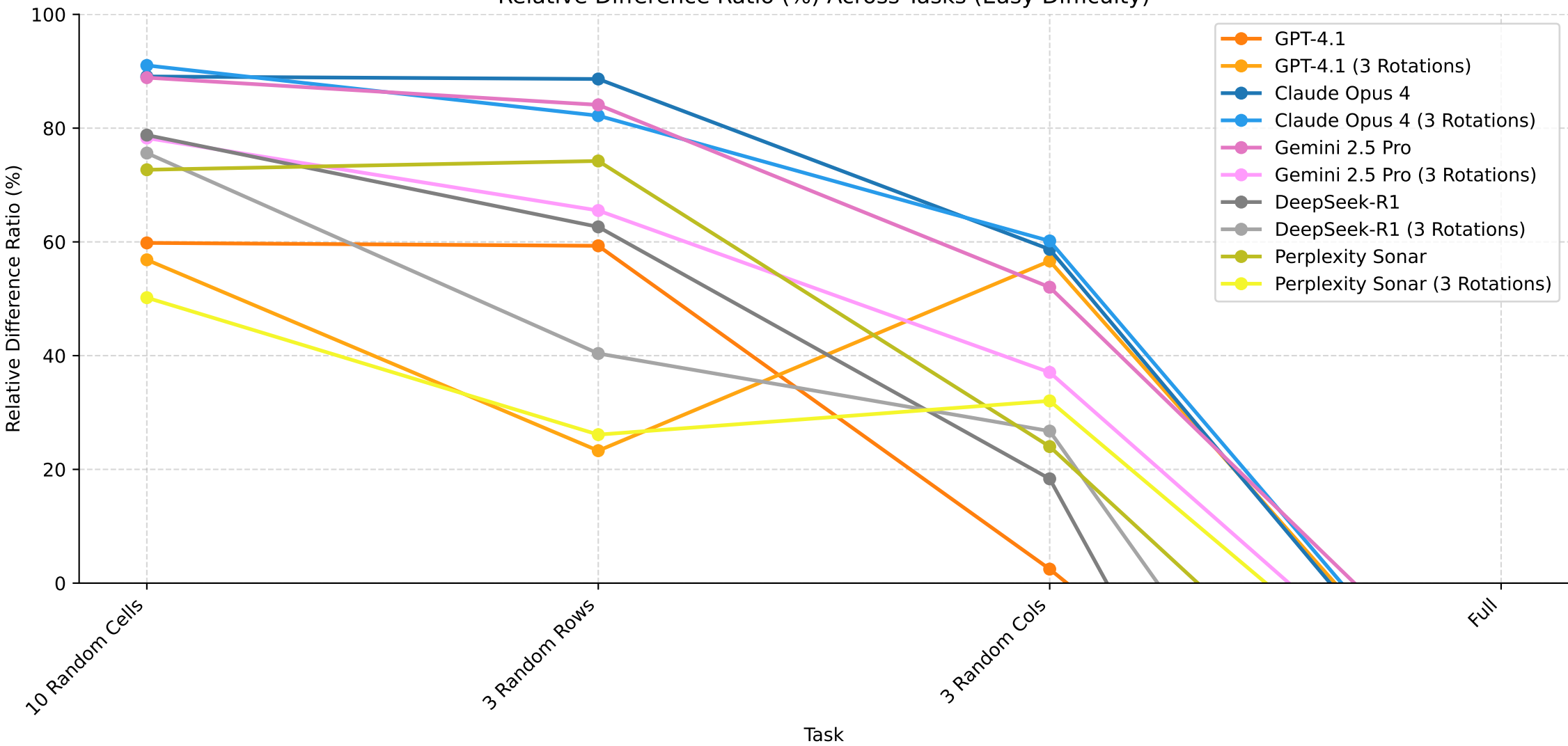
Relative Difference Ratio (%) Across Tasks (Easy Difficulty)
