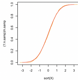
pvalue(shapiro)= 0.2
