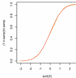
pvalue(shapiro)= 0.04
