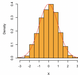
pvalue(shapiro)= 0.2
