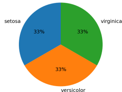
Variable qualitative : proportions
