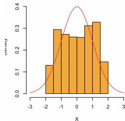
pvalue(shapiro)= 0
