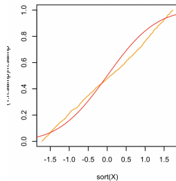
pvalue(shapiro)= 0
