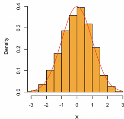
pvalue(shapiro)= 0.04
