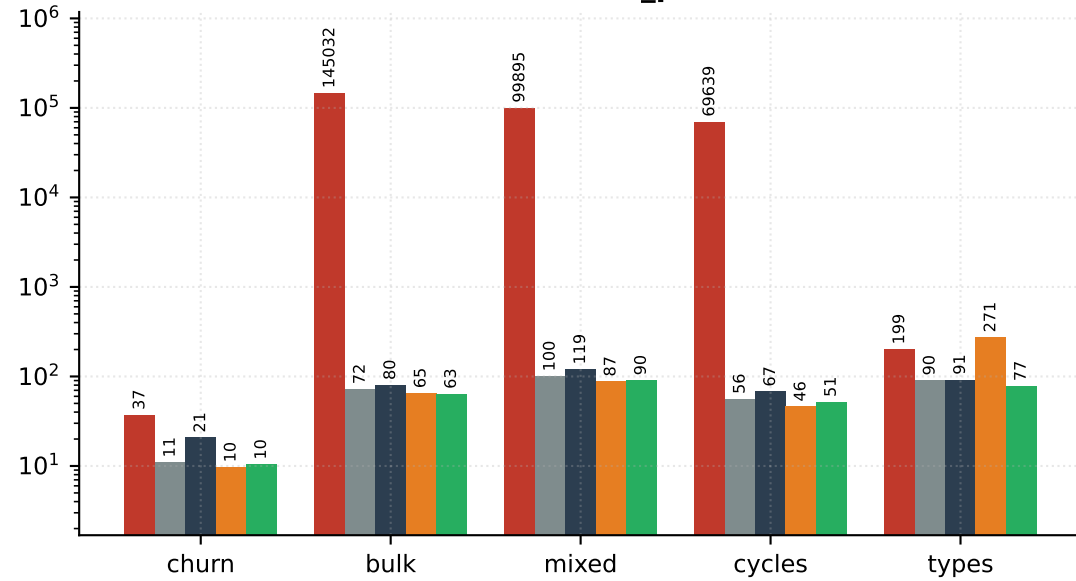
std::shared_ptr
