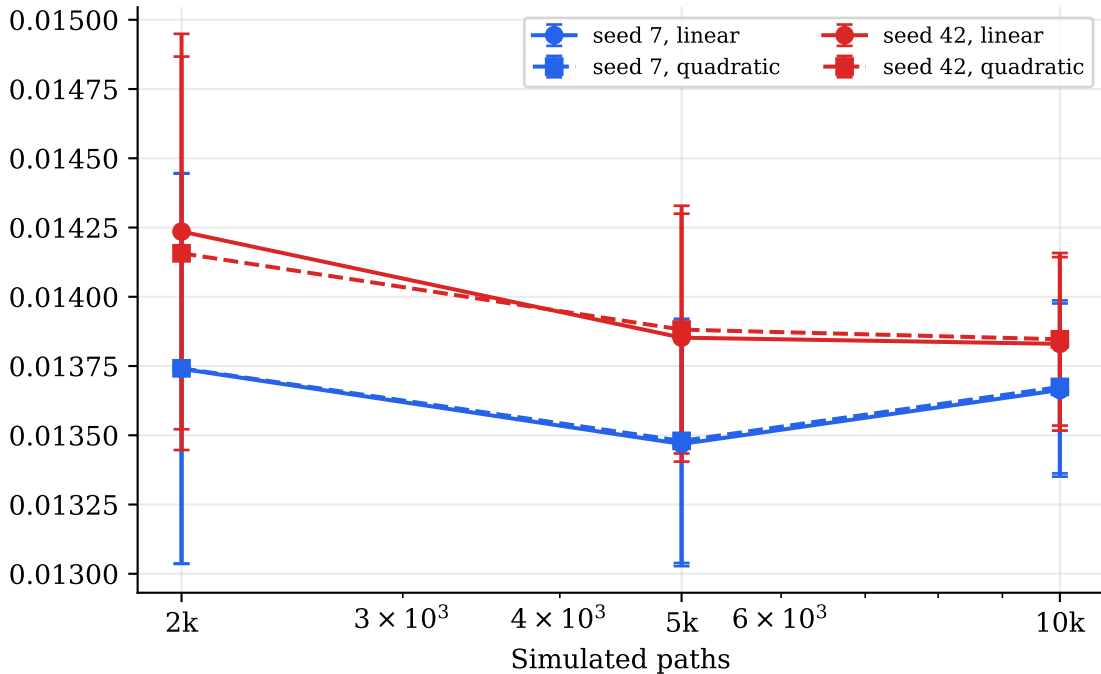
Bermudan swaption price
