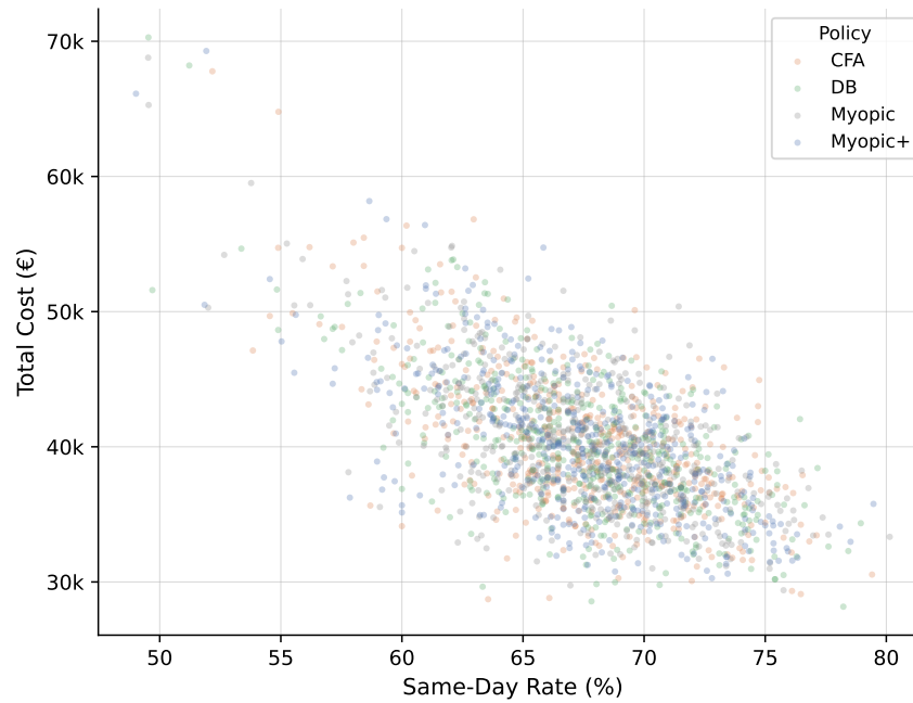
Figure 6: Same-day rate versus total cost for all individual runs under centrality-based zone selection. Each point represents one Monte Carlo run; color indicates policy.
