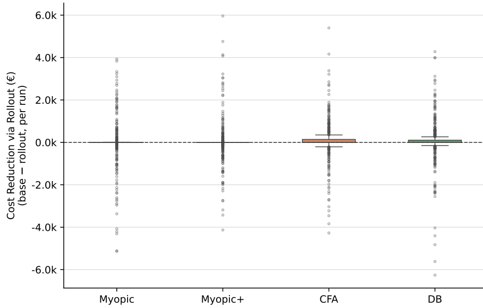
Figure 9: Paired cost reduction (base minus rollout) per run for each policy. Positive values indicate the rollout lowered cost. Dashed line marks zero. All variants use value-based zone selection (500 runs each).
