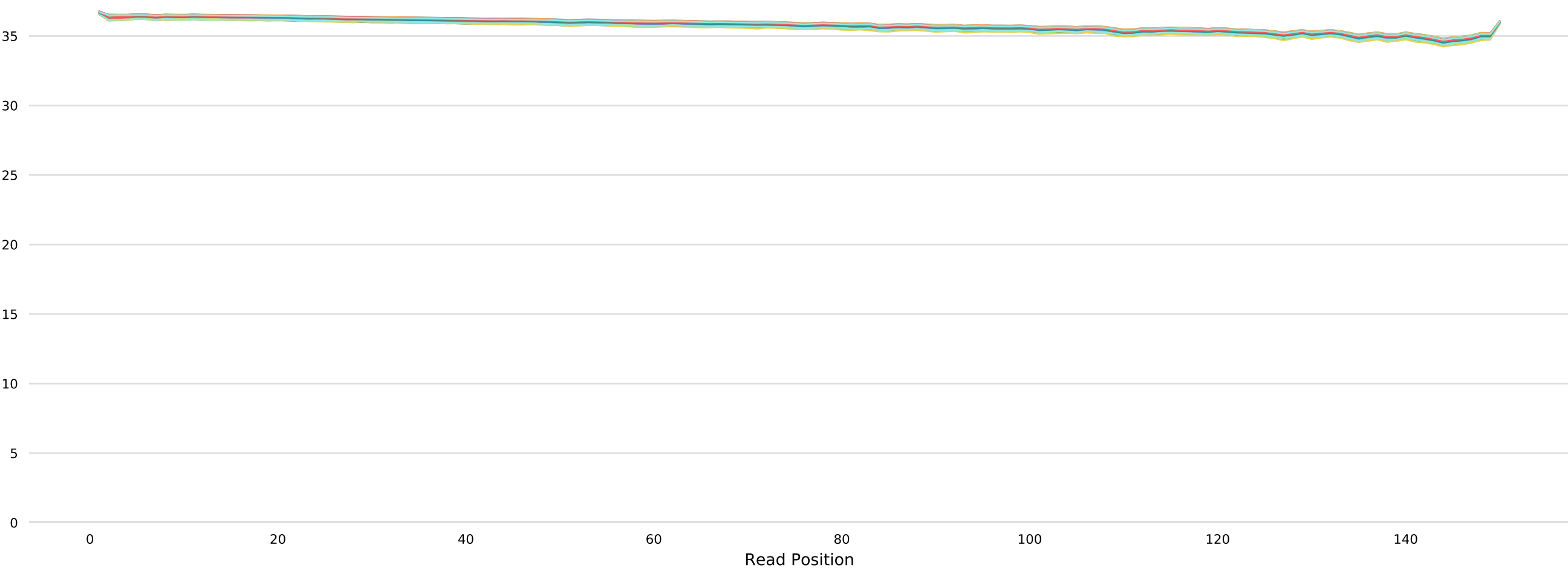
Fastp: Sequence Quality
