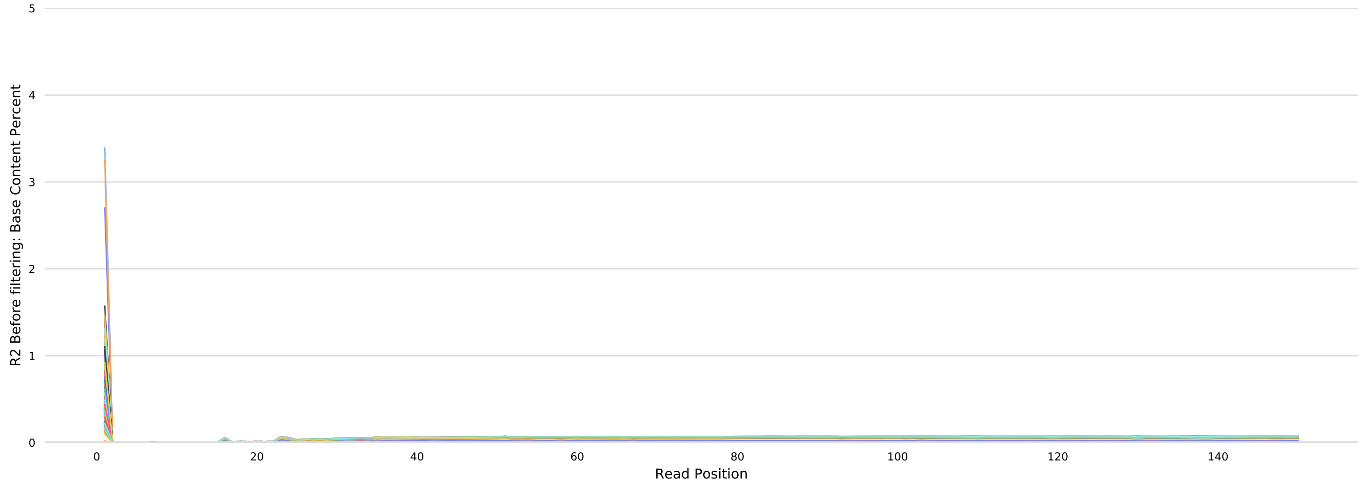
Fastp: Read N Content
