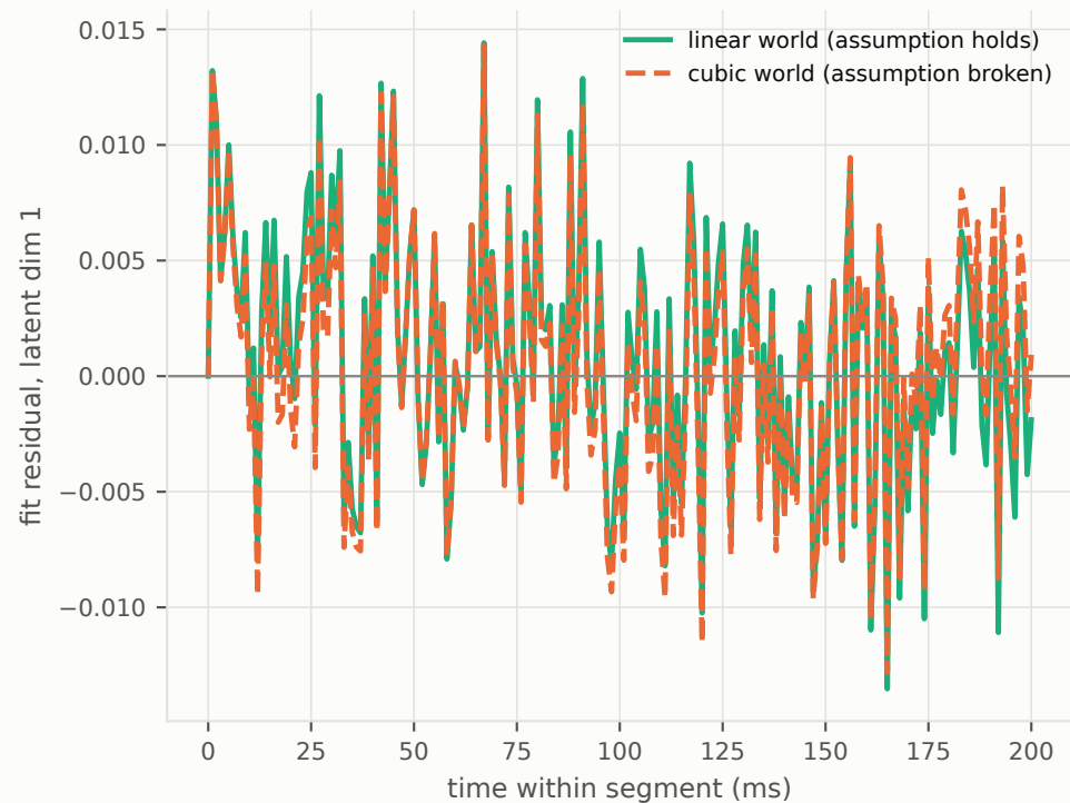
Residual structure is the only warning you get
