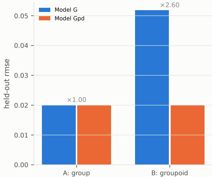
Held-out error by model and world
