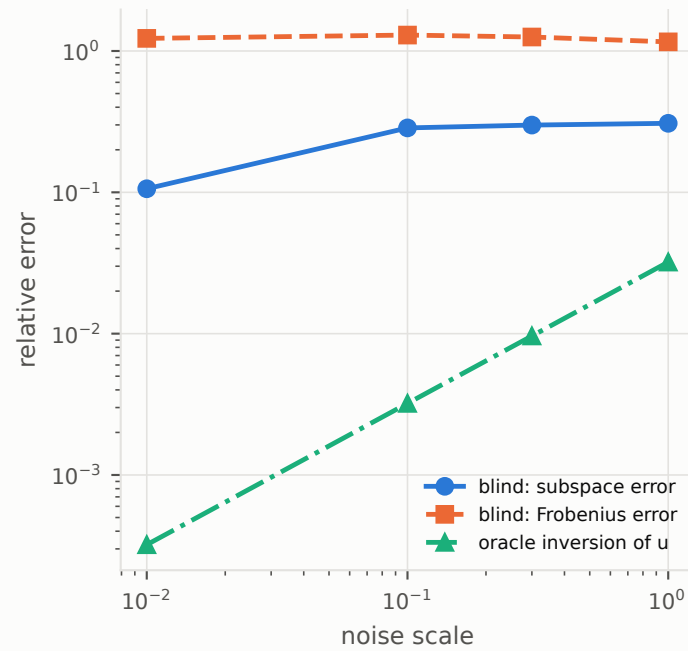
What each estimator can reach
