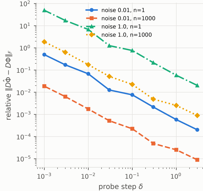
Noise and averaging, quadratic \Phi
