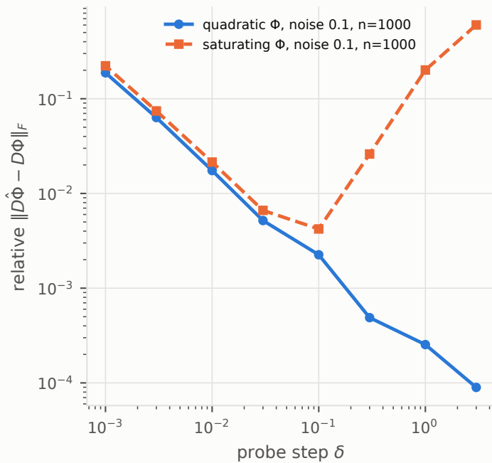
Probe Jacobian: bias appears only with curvature
