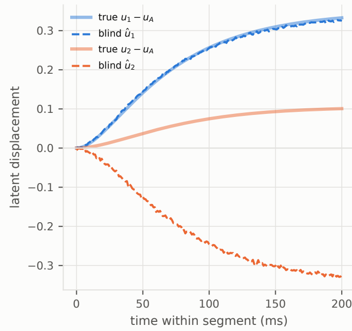
Blind inversion recovers a rotated latent
