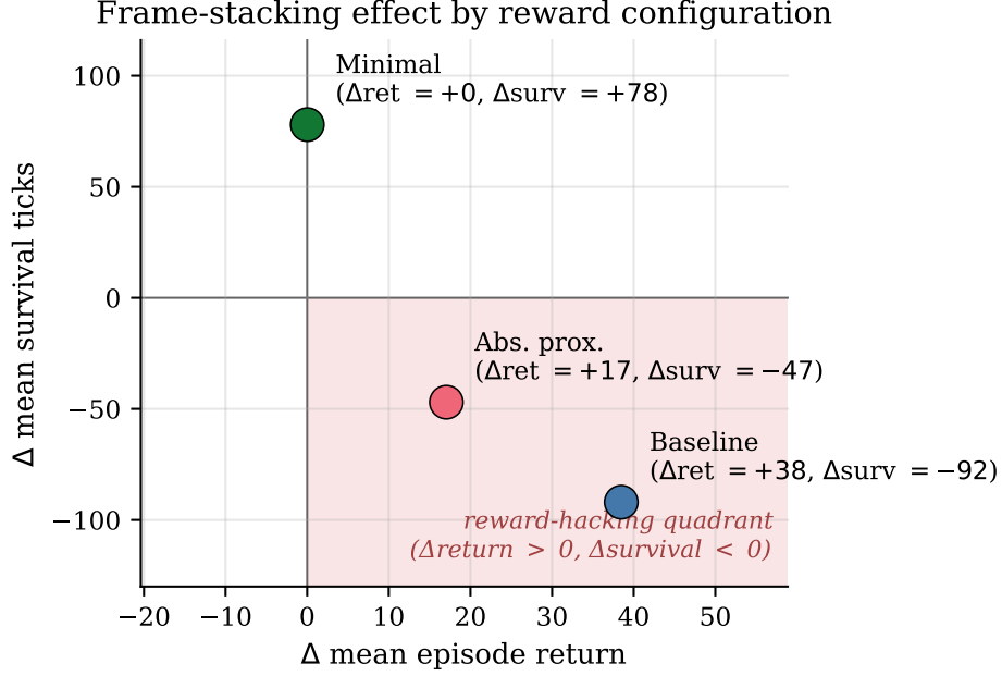
Figure 4: Frame-stacking effect on mean episode return (x-axis) and mean survival ticks (y-axis), one point per reward configuration. Each point is the (sf \rightarrow fs) shift in the per-cell means, averaged across the four training seeds and 100 evaluation worlds. The shaded lower-right region marks the reward-hacking quadrant where return rises and survival falls.
