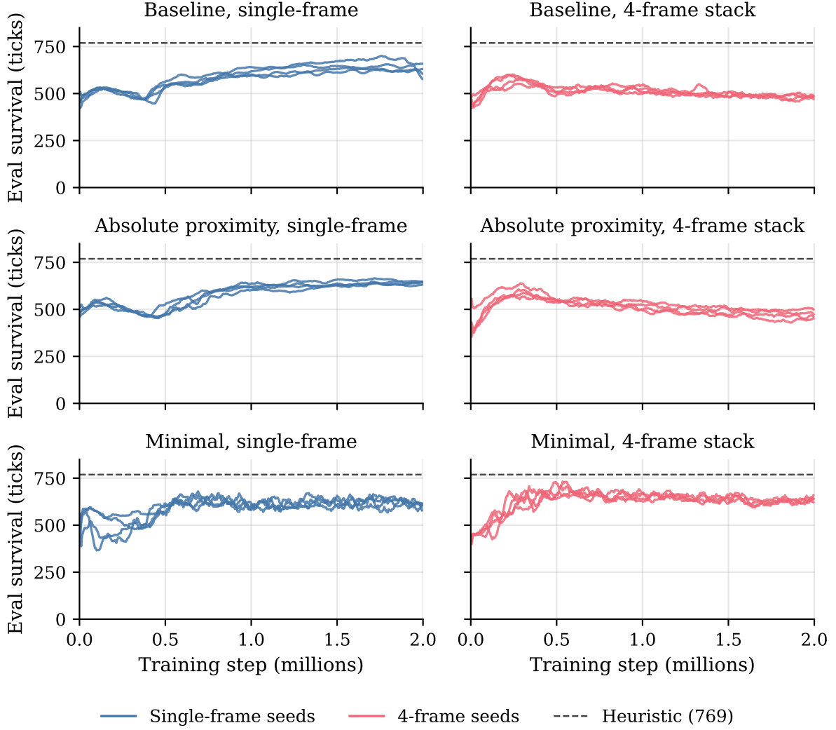
Figure 7: In-training evaluation survival vs training step for the six ablation cells. Each line is one seed, smoothed with a 10-eval rolling mean (50,000-step window). The dashed gray line at 769 ticks marks the heuristic baseline.
