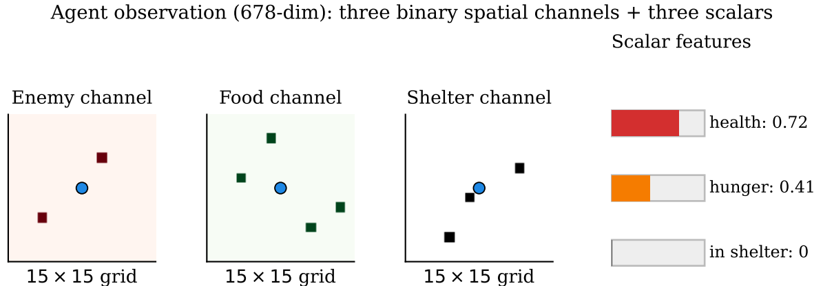
Figure 2: Observation structure. The agent (blue dot at the window center) sees three binary 15 \times 15 grids corresponding to enemy, food, and shelter presence within radius 7, plus three scalar features summarizing the agent's internal state. Section 6.5 crosses this single-frame observation with a 4-frame stacked variant (12 spatial channels) as the observation-side ablation.
