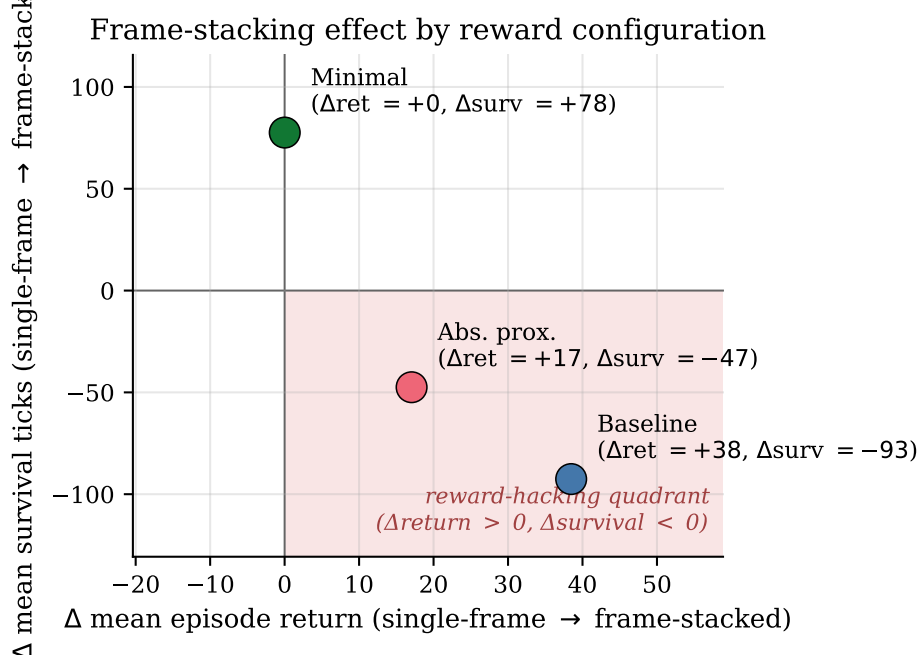
Figure 4: Frame-stacking effect on mean episode return (x-axis) and mean survival ticks (y-axis), one point per reward configuration. Each point is the (sf \rightarrow fs) shift in the per-cell means, averaged across the four training seeds and 100 evaluation worlds. The shaded lower-right region marks the reward-hacking quadrant where return rises and survival falls.
