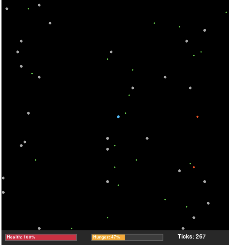
Figure 1: Screenshot of the survival environment. The agent (blue dot) is near the grid center. Two enemies (red dots) are visible to the east. Food items (small green dots) are scattered across the grid and replenish stochastically over time. Shelters (large gray dots) are placed once at episode start and remain fixed. The bottom bar reports current health and hunger, and current tick count.
