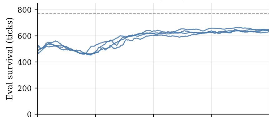
Engineered V5, single-frame
