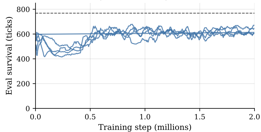
Engineered V5, single-frame
