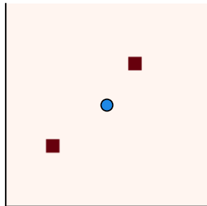
Enemy channel
