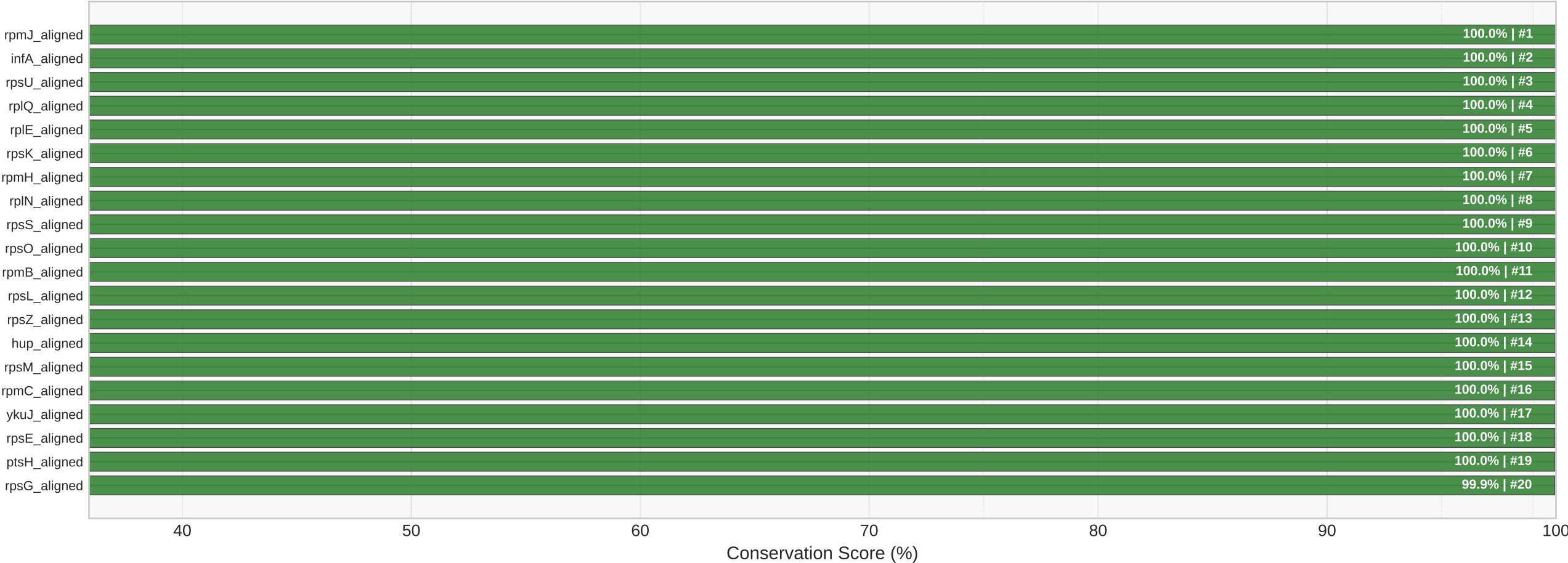
Top 20 Most Conserved Core Genes
