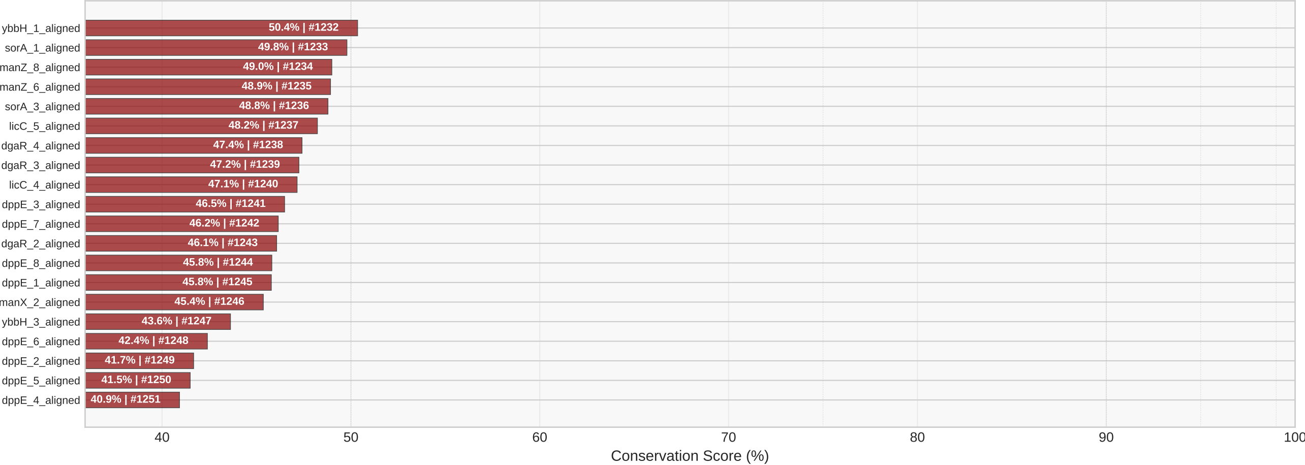
Bottom 20 Least Conserved Core Genes
