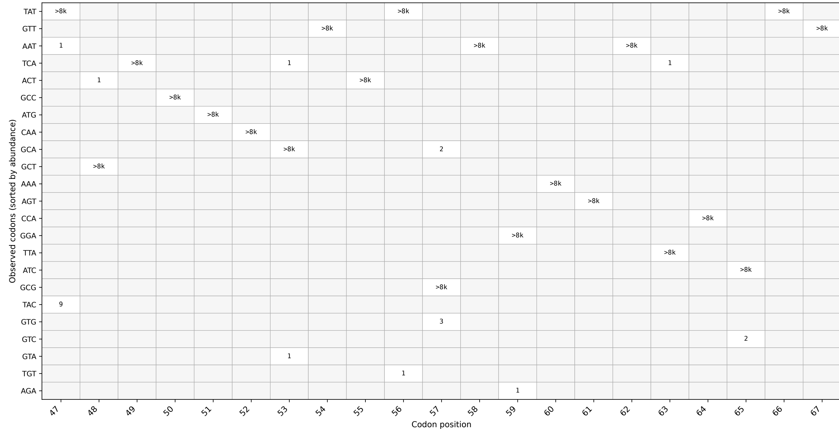
frpC: codon usage around position 57 (window 47–67)
