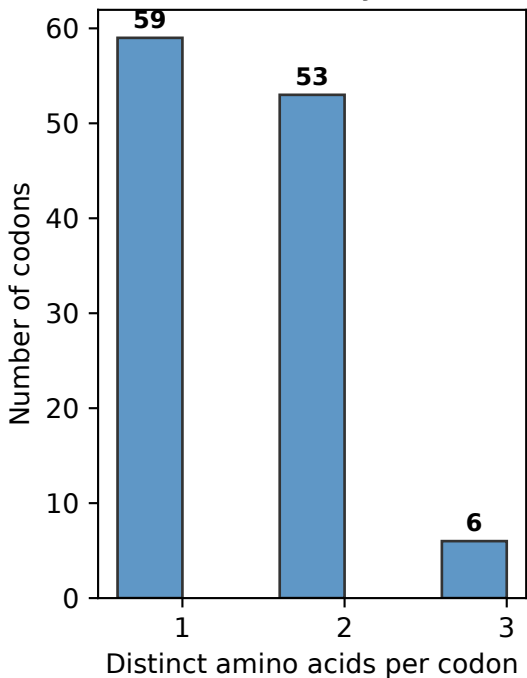
fA2: amino-acid diversity in variable
