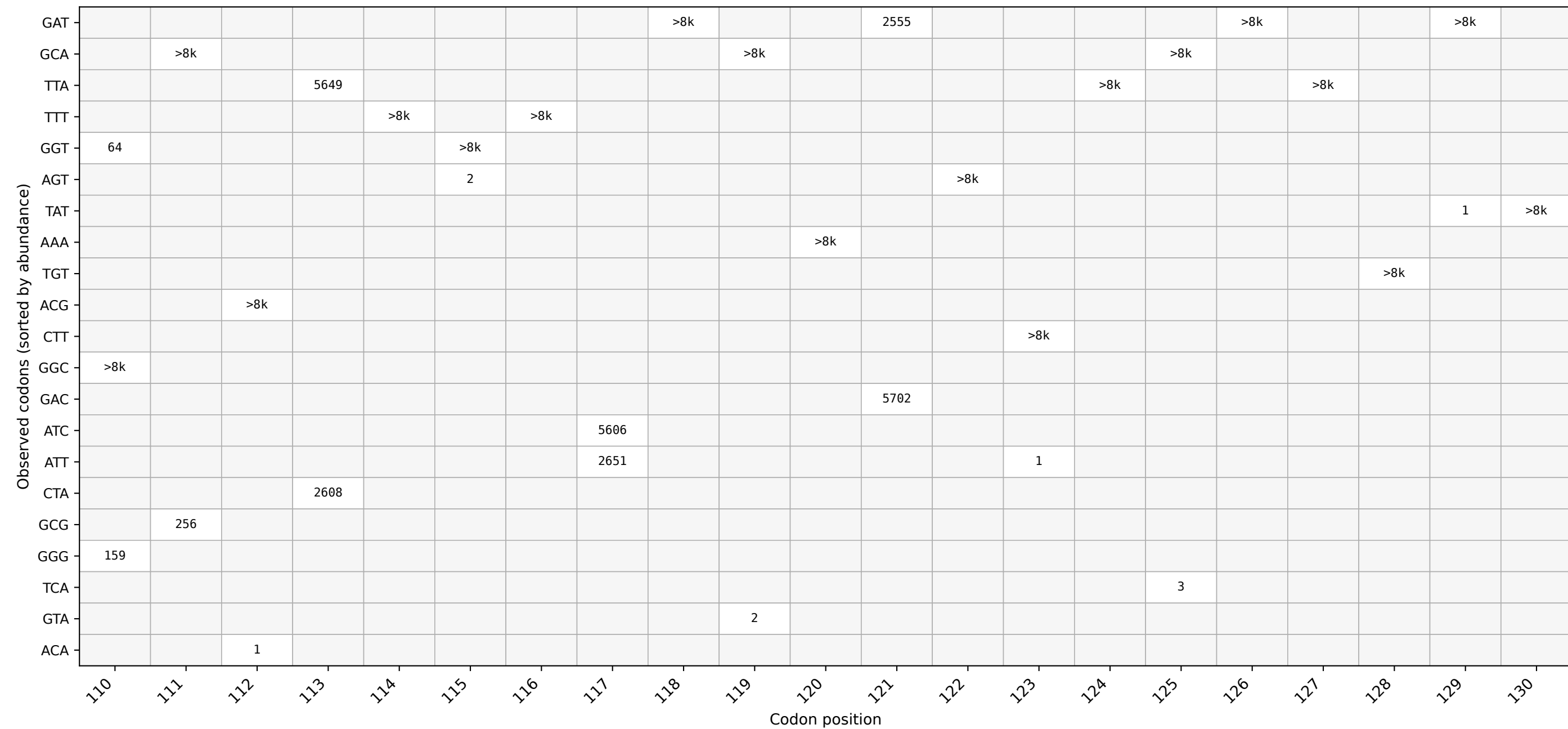
frpC: codon usage around position 120 (window 110-130)
