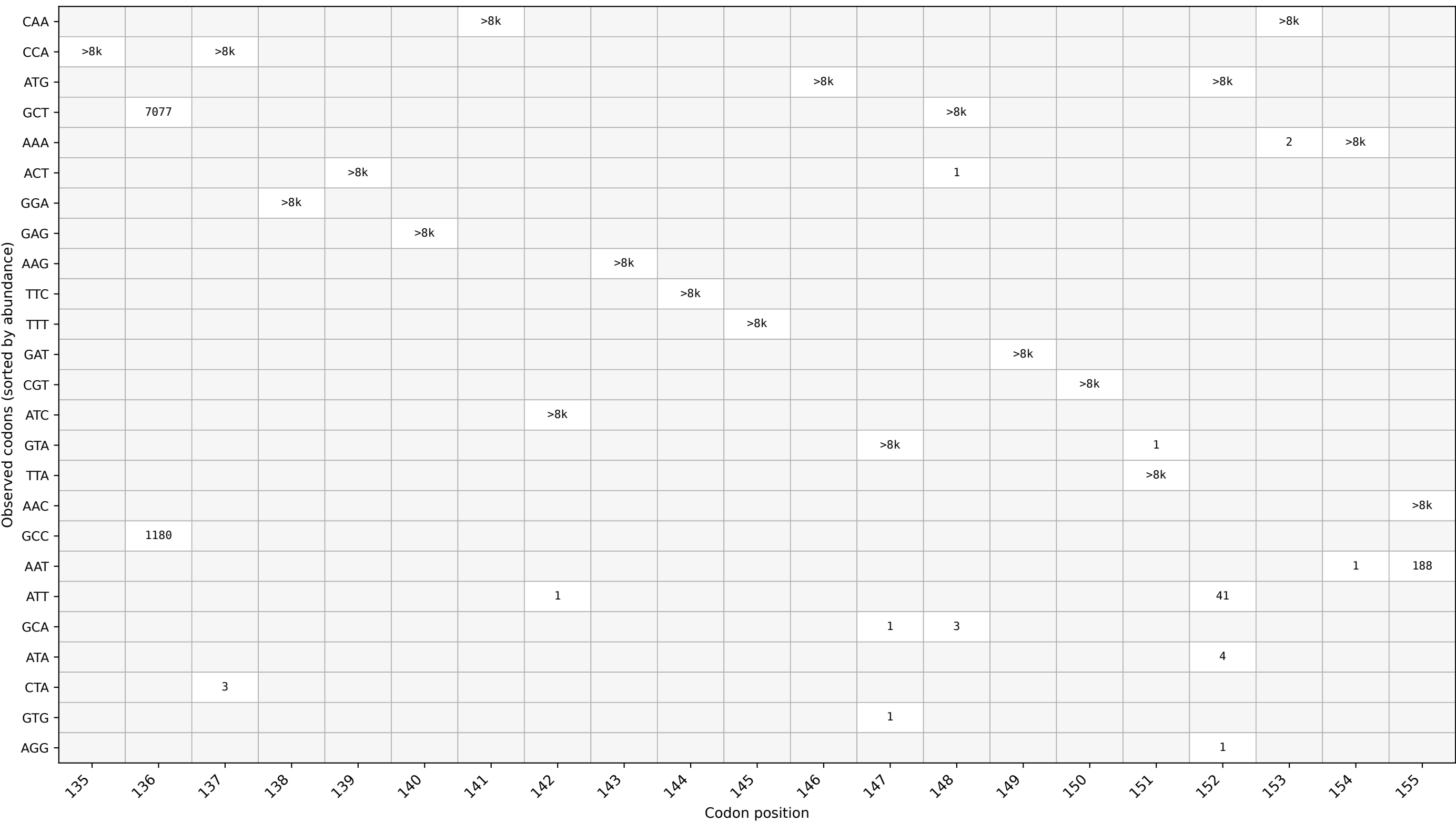
frpC: codon usage around position 145 (window 135-155)
