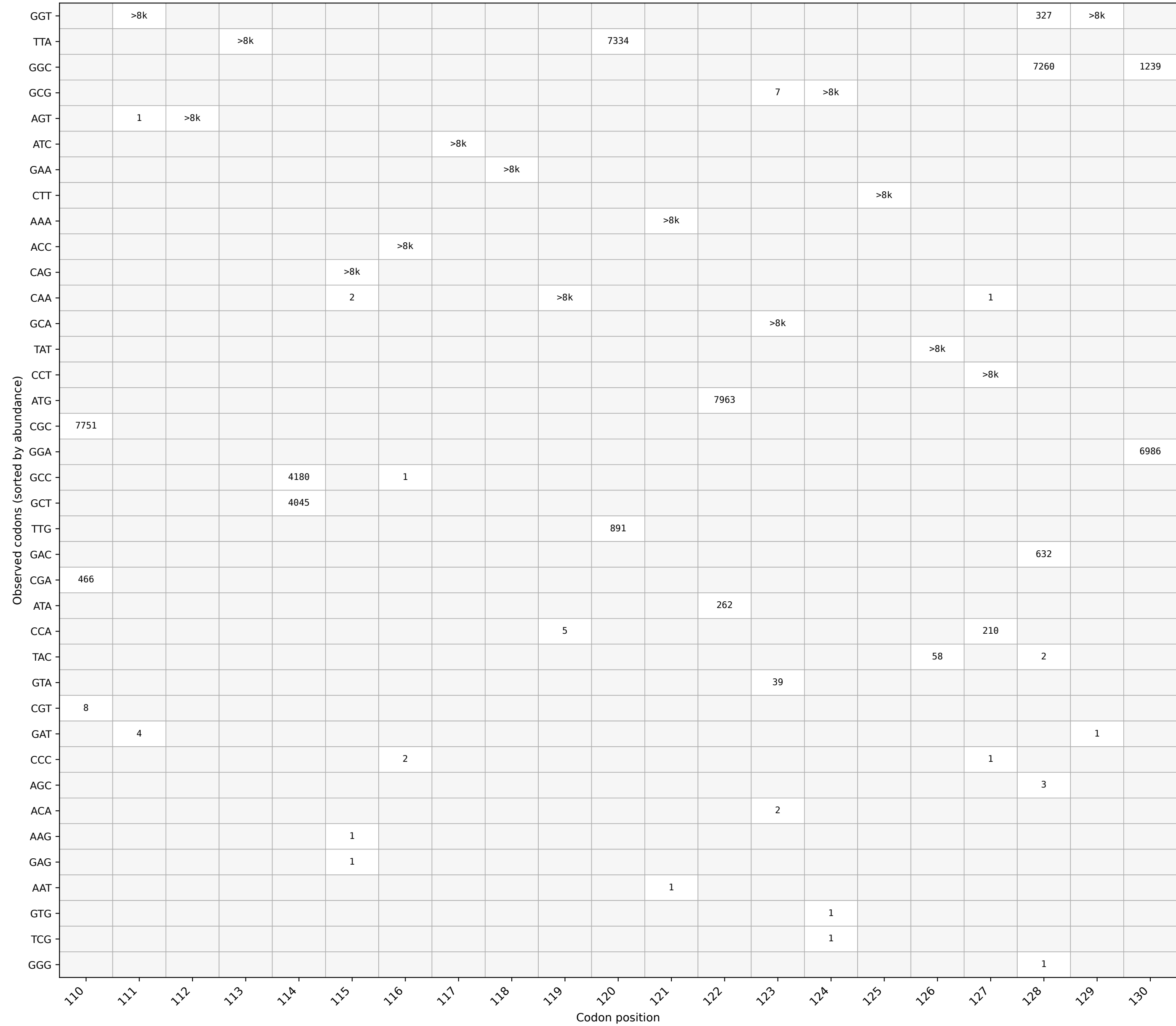
fruR: codon usage around position 120 (window 110-130)
