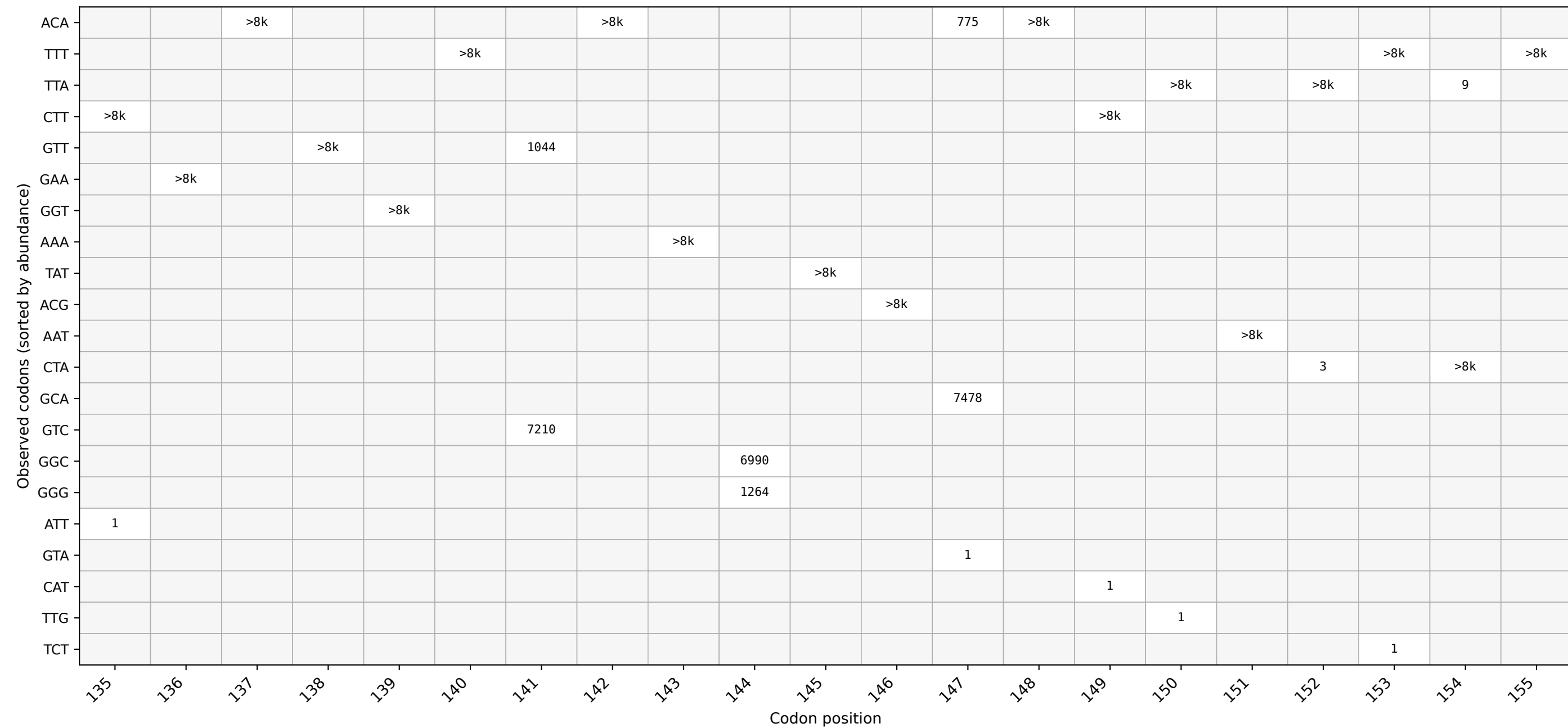
glpC: codon usage around position 145 (window 135-155)
