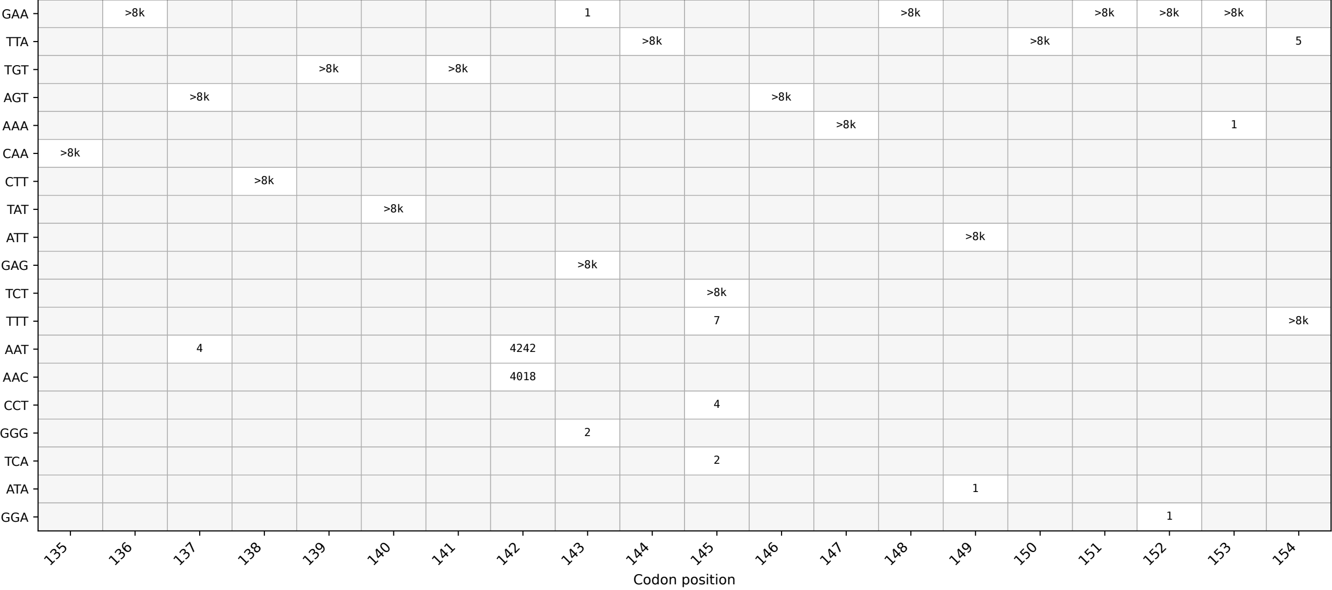
ptsA: codon usage around position 145 (window 135-154)
