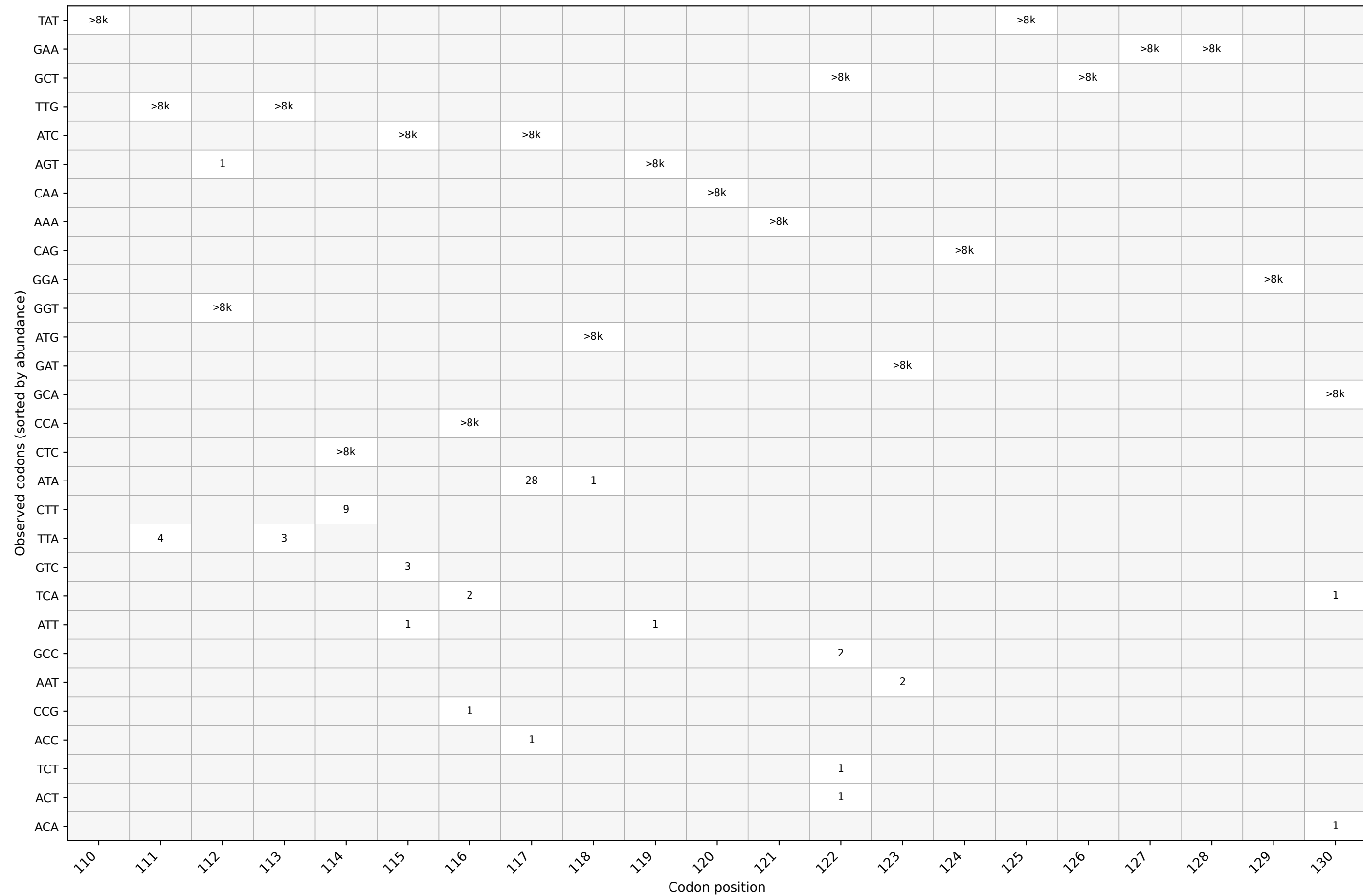
ptsC: codon usage around position 120 (window 110-130)
