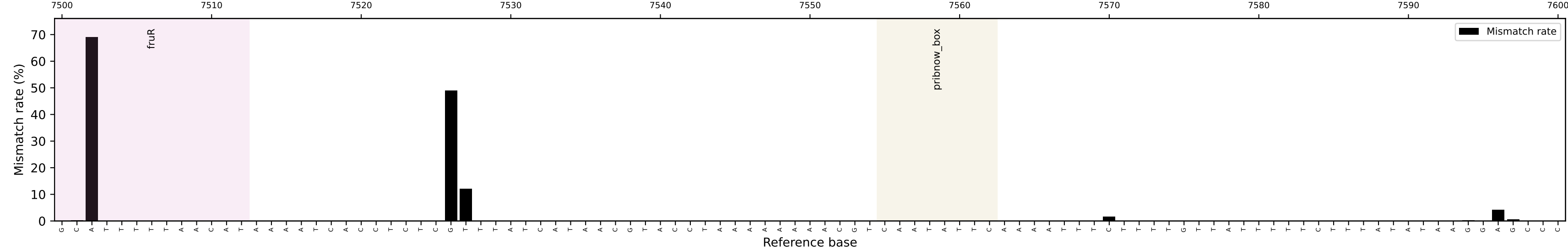
Mismatch rate along operon (Legacy) (positions 7500-7600)
