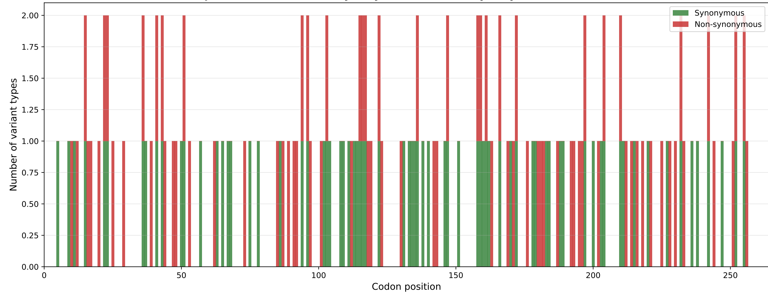
ptsC - Distribution of Synonymous and Non-synonymous Variation
