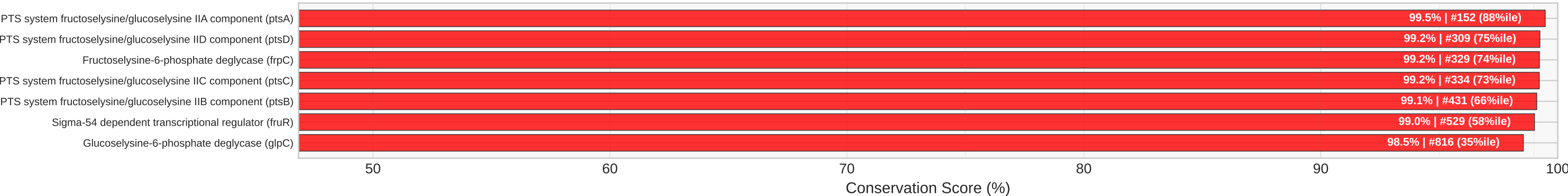
Fructoselysine/Glucoselysine Operon Genes
