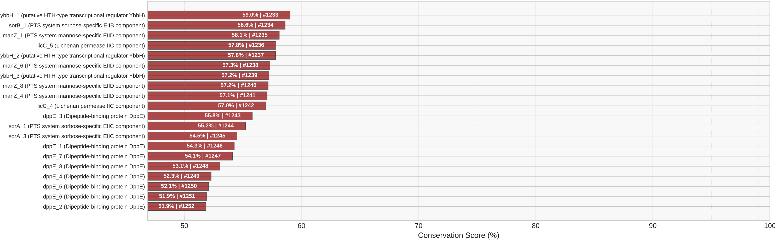
Bottom 20 Least Conserved Core Genes
