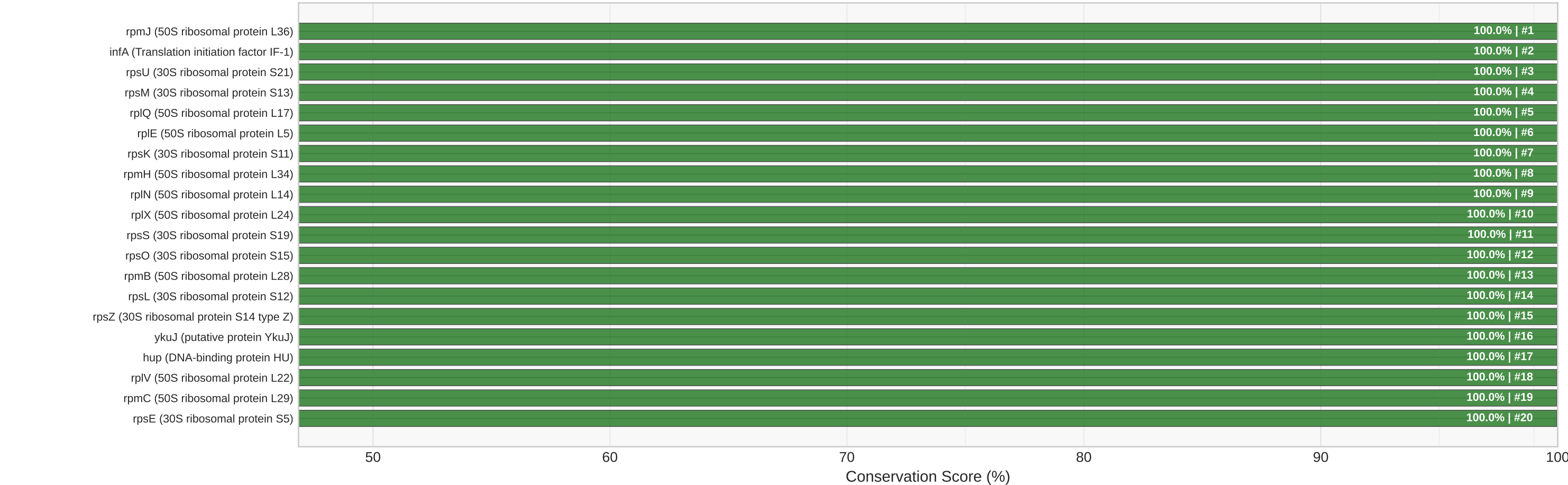
Top 20 Most Conserved Core Genes
