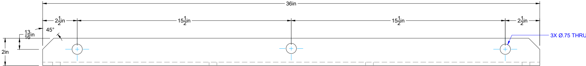
Front View Rigging Angle 2 x 2 x 1/4 - Make Qty.2 Scale = 1:4
