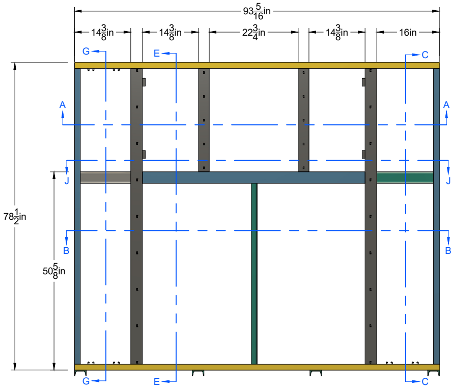
Front View Steel Framing Assembly Scale = 1:25
