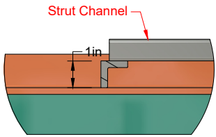
DETAIL D: 1in Angle SCALE 1:5
