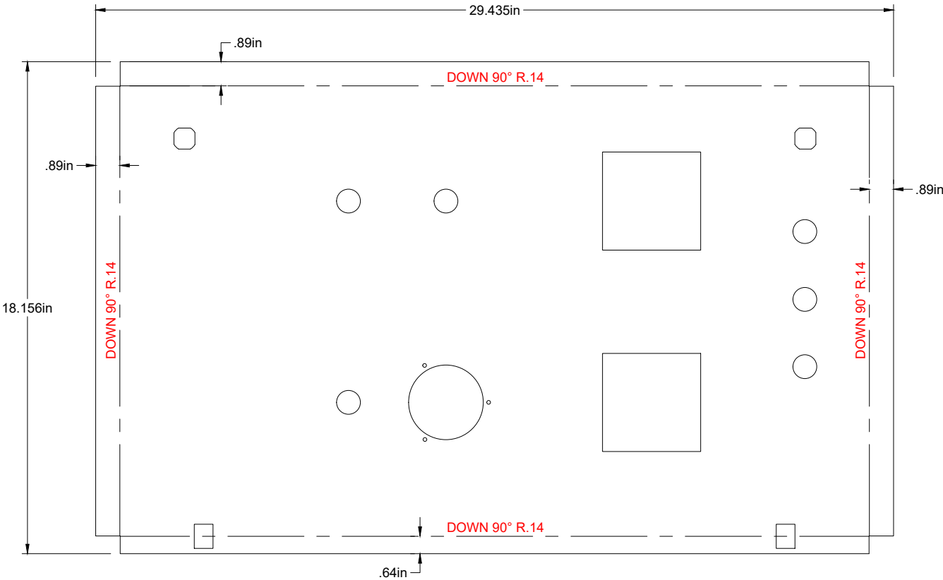
Flat Pattern TRD (x1) 12 ga Steel Scale = 1:8
