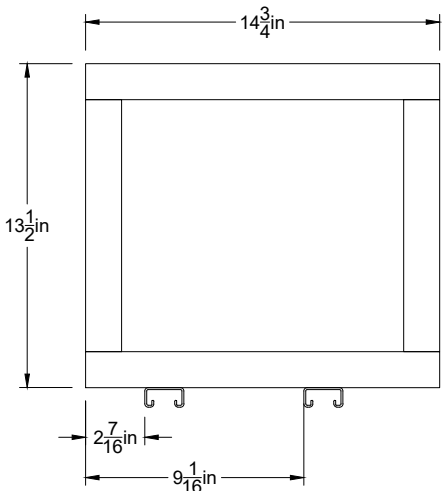
Front View Vert. Distribution Rack B1 Scale = 1:10
