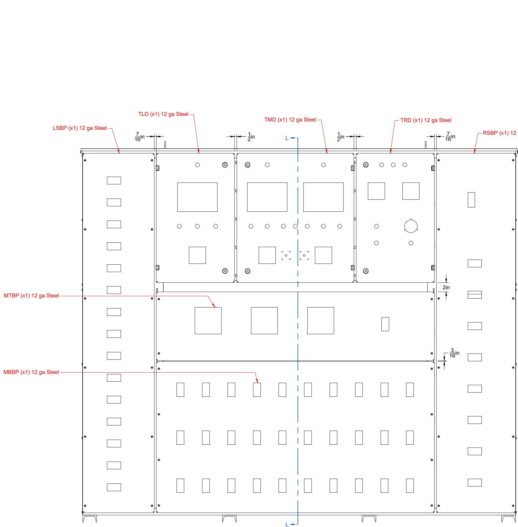
Front View Josh David Espers 50 BRK 480 Scale = 1:12
