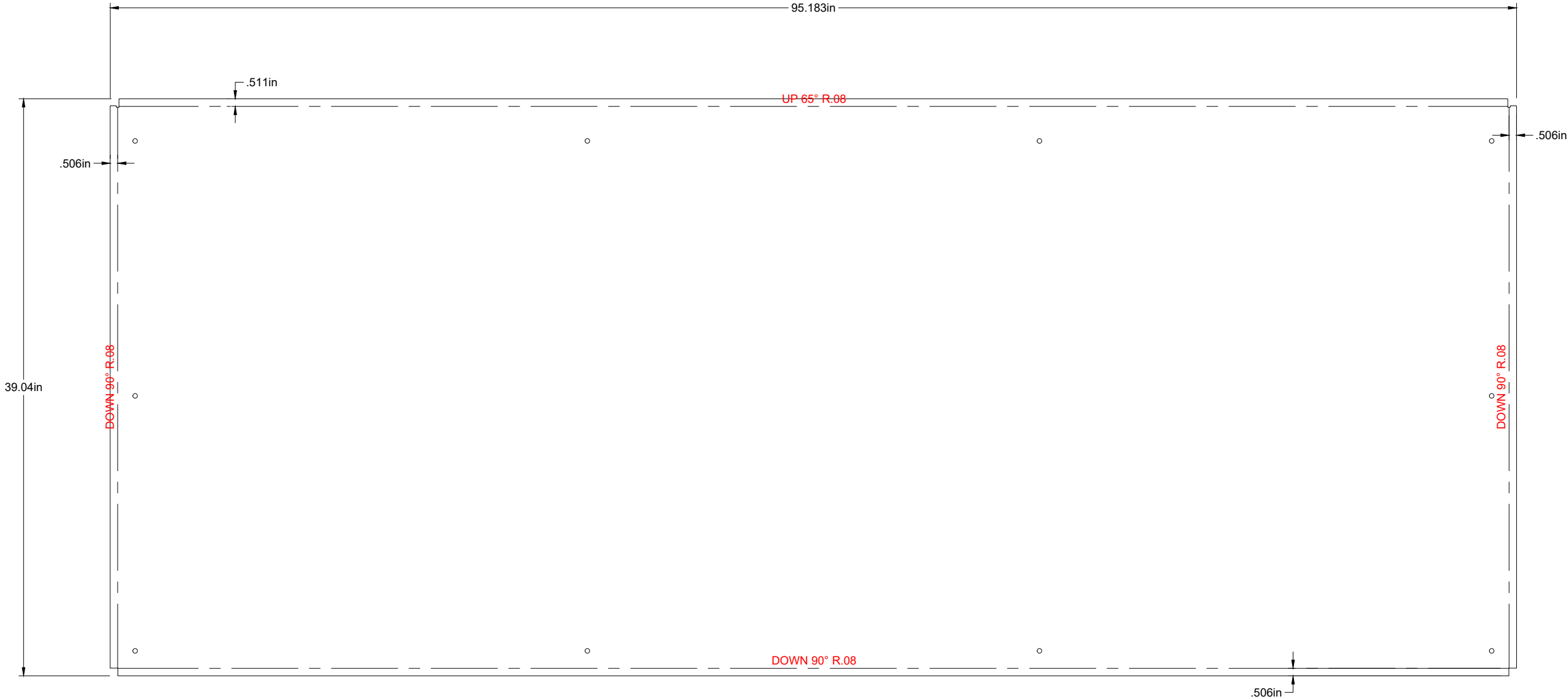
Flat Pattern TC (x1) 14 ga Steel Scale = 1:8
