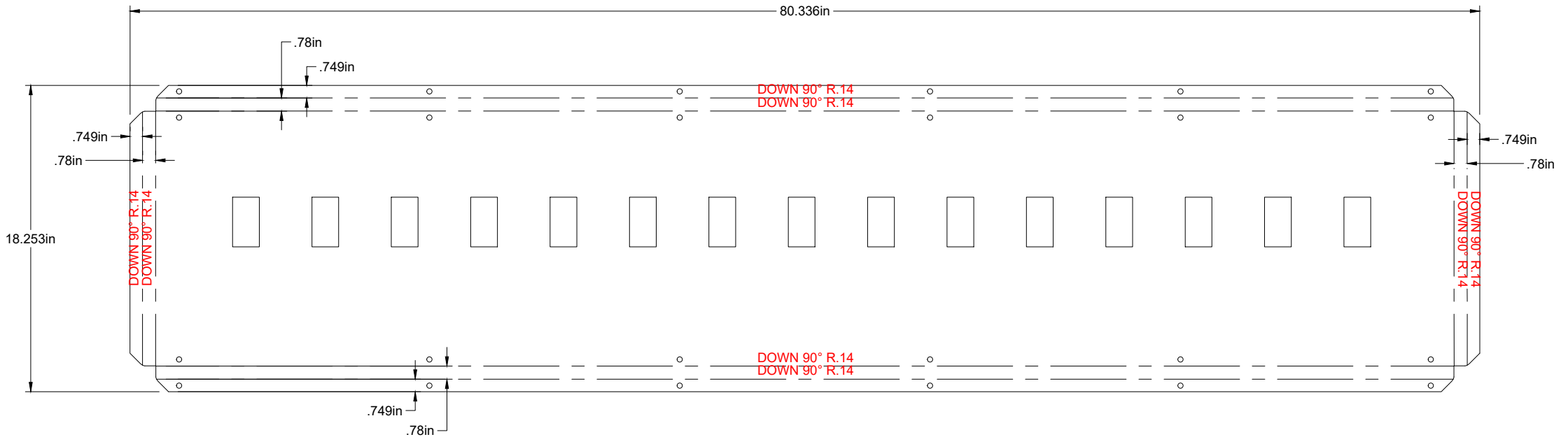
Flat Pattern LSBP (x1) 12 ga Steel Scale = 1:8
