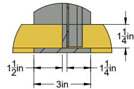
DETAIL S: Cust. T Slot Layout SCALE 1:5
