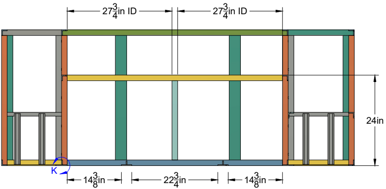
SECTION J-J SCALE 1:25
