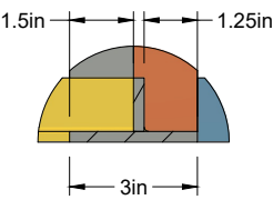
DETAIL K: Cust. T (Not Sym) Adjacent Side Mirrored SCALE 1:5
