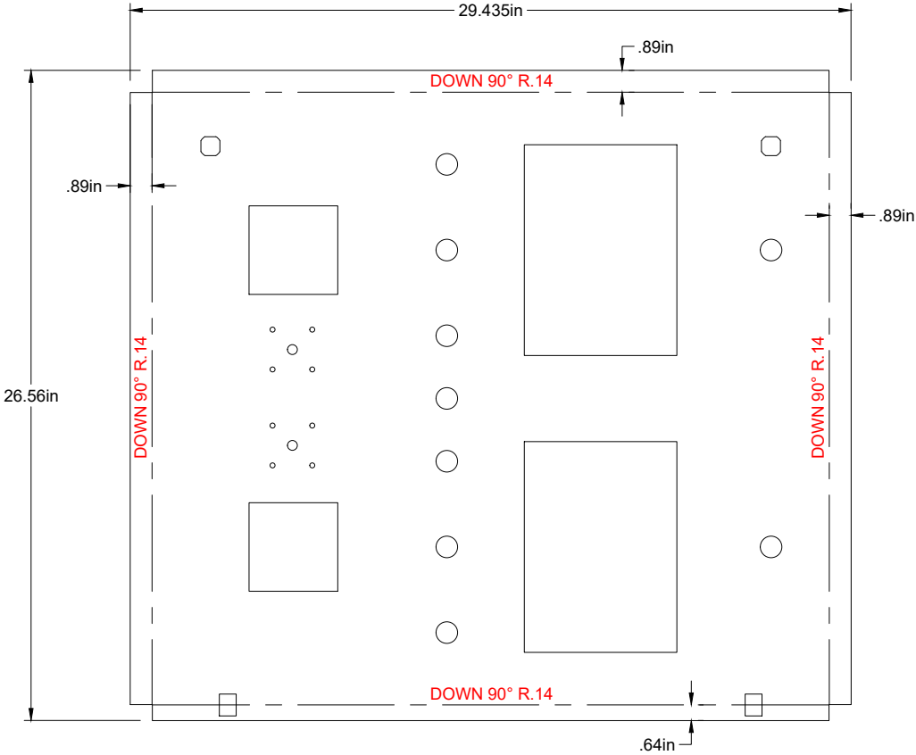
Flat Pattern TMD (x1) 12 ga Steel Scale = 1:8
