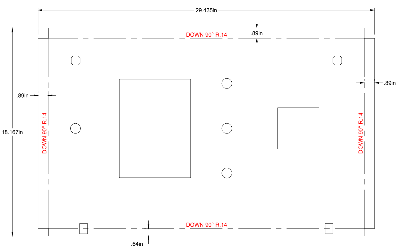
Flat Pattern TLD (x1) 12 ga Steel Scale = 1:8
