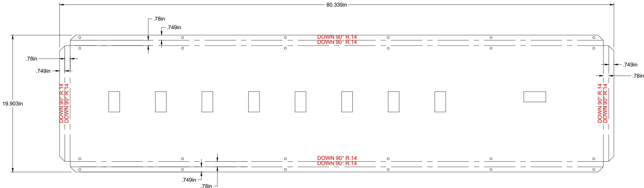
Flat Pattern RSBP (x1) 12 ga Steel Scale = 1:8
