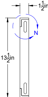
Side View Horz. Distribution Rack B Scale = 1:10
