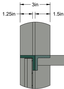
DETAIL I SCALE 1:5
