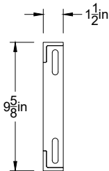
Side View Horz. Distribution Rack A - Make Qty.3 Scale = 1:10
