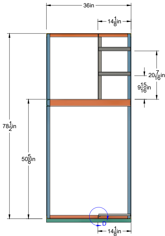
SECTION C-C SCALE 1:25
