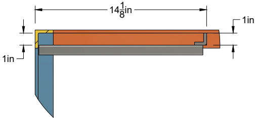
DETAIL H SCALE 1:8
