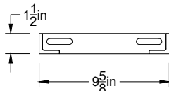
Top View Vert. Distribution Rack B Scale = 1:10
