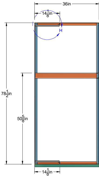
SECTION G-G SCALE 1:25
