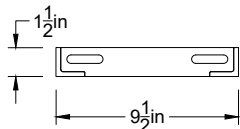
Top View Vert. Distribution Rack A Scale = 1:10
