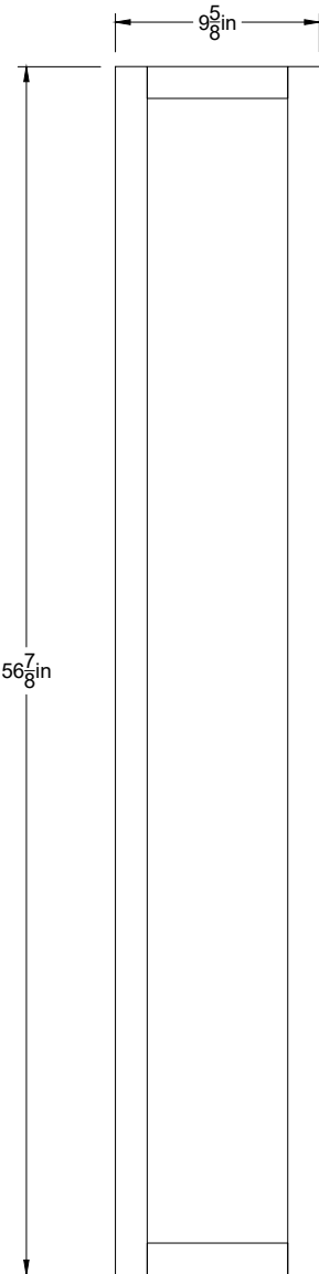
Front View Vert. Distribution Rack B Scale = 1:10
