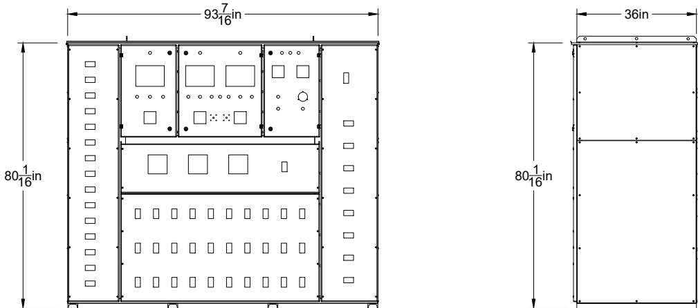
Front View Josh David Espers 50 BRK 480 Scale = 1:40
