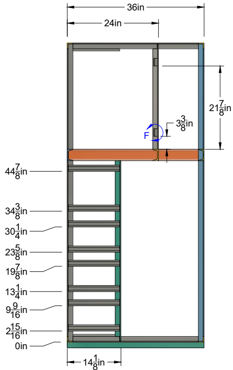
SECTION E-E SCALE 1:25
