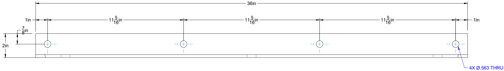
Top View Rigging Angle 2 x 2 x 1/4 - Make Qty.2 Scale = 1:4
