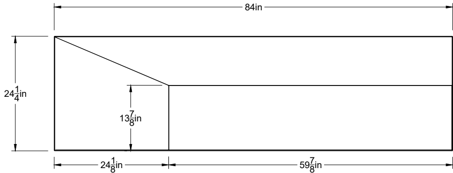
Bottom View Inlet Adapter Scale = 1:20
