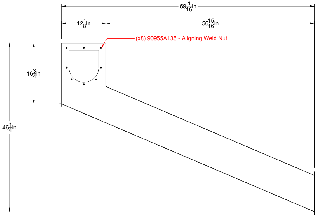
Front View Duct Unit2-A Scale = 1:16
