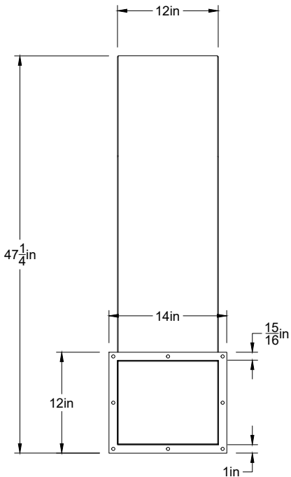
Right View Duct Unit2-A Scale = 1:16
