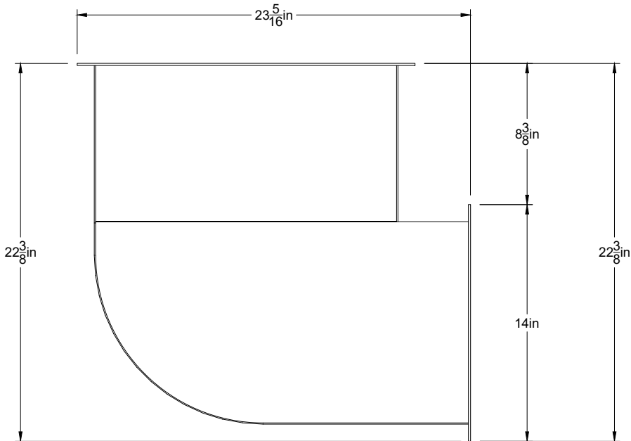
Top View Duct Unit2-B Scale = 1:8
