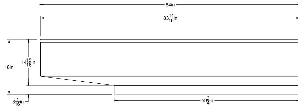
Front View Inlet Adapter Scale = 1:16
