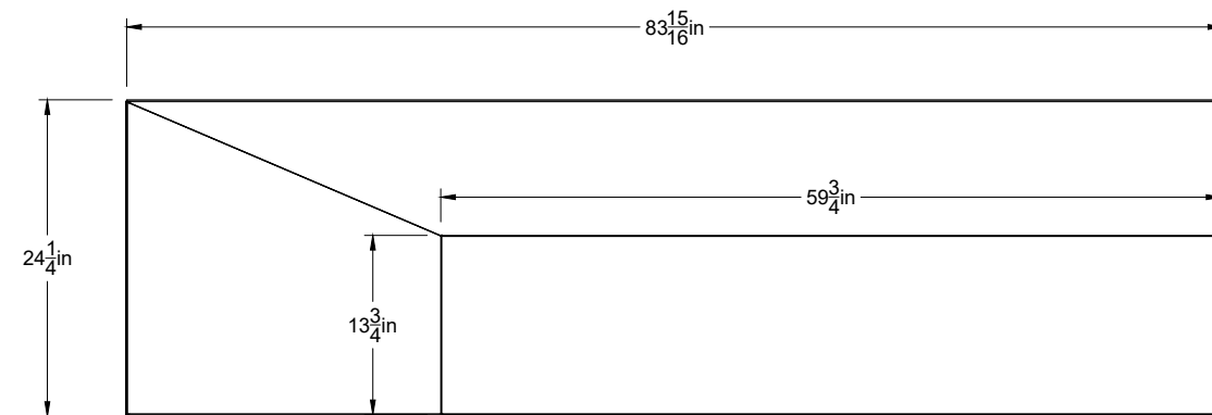
Bottom View Inlet Adapter Scale = 1:16
