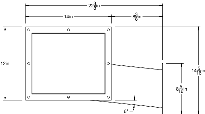
Right View Duct Unit2-B Scale = 1:8
