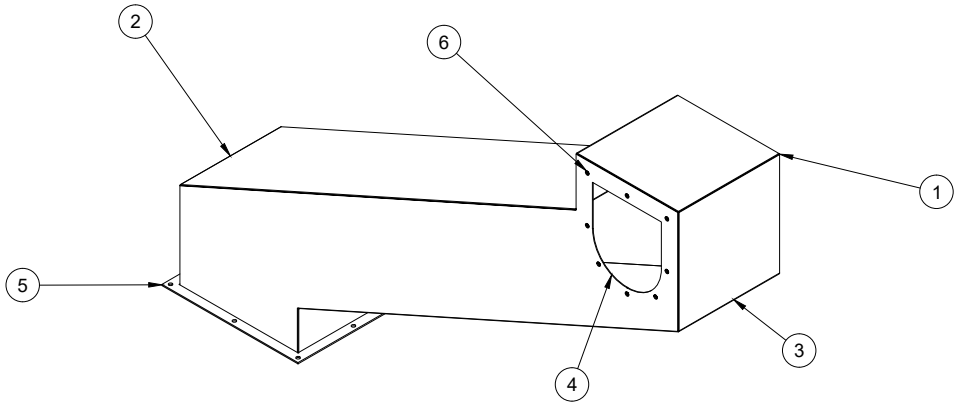
ISO Duct Unit1 Scale = Perspective
