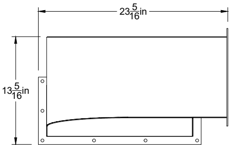
Front View Duct Unit 2-B Scale = 1:12
