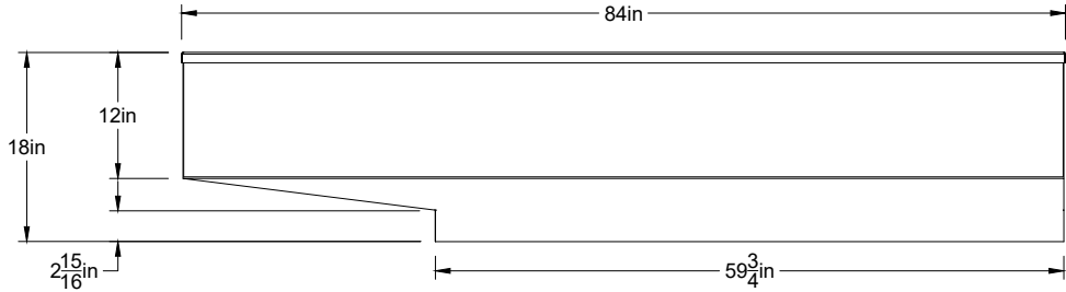
Front View Inlet Adapter Scale = 1:20
