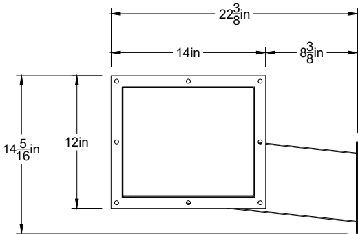
Right View Duct Unit 2-B Scale = 1:12
