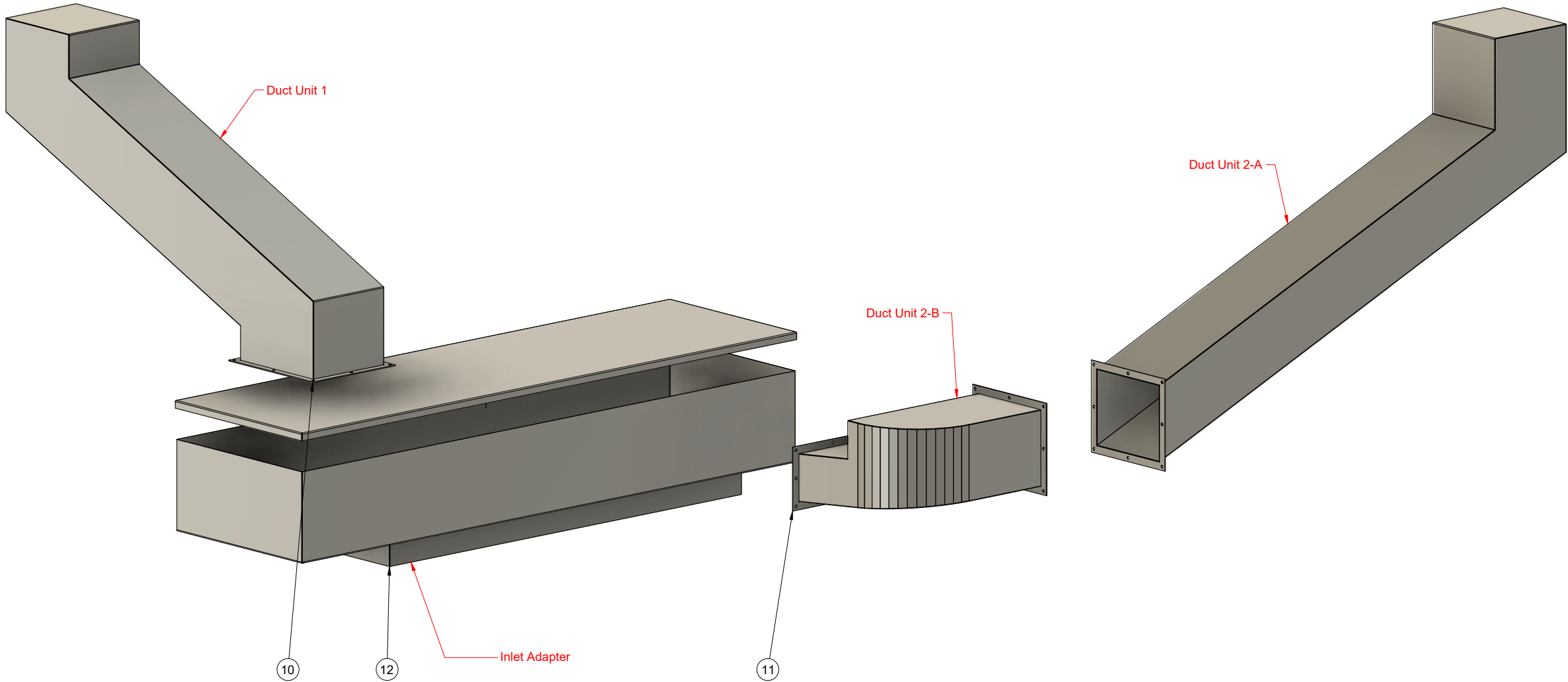
EXP ISO Ice Maker Transition - Duct Assembly Scale = Perspective
