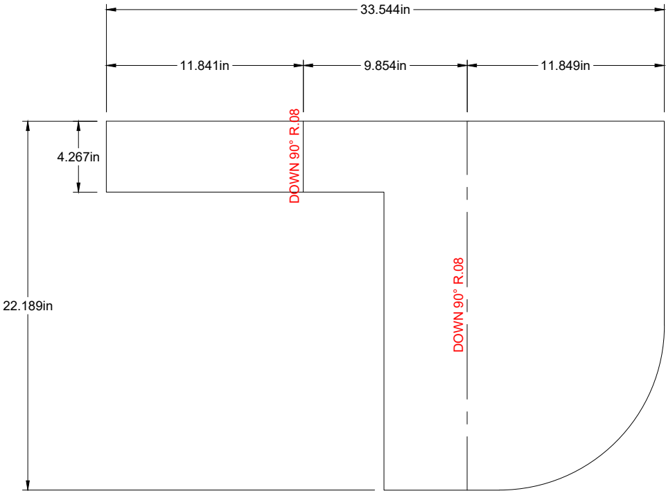
Flat Pattern U2TP (x1) 14 ga Stainless Scale = 1:8
