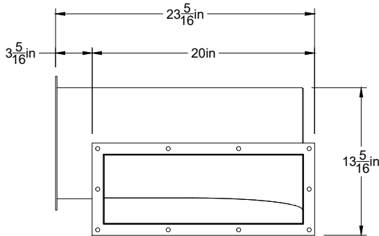
Back View Duct Unit 2-B Scale = 1:12
