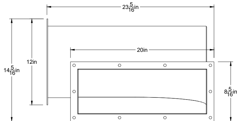
Back View Duct Unit2-B Scale = 1:8
