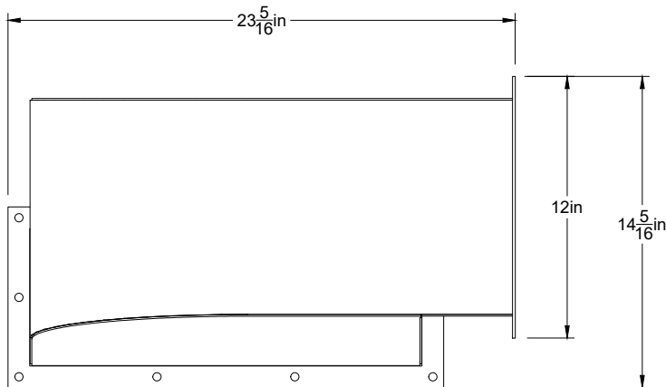
Front View Duct Unit2-B Scale = 1:8
