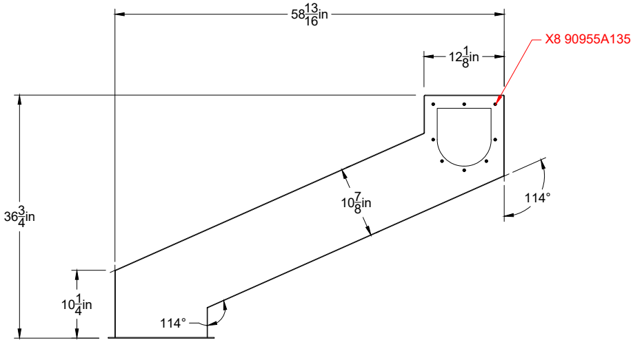
Front View Duct Unit 1 Scale = 1:20
