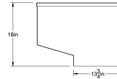
Right View Inlet Adapter Scale = 1:16
