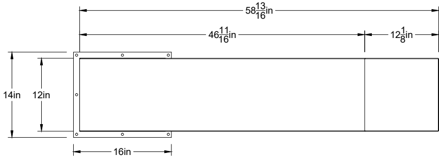
Top View Duct Unit1 Scale = 1:16
