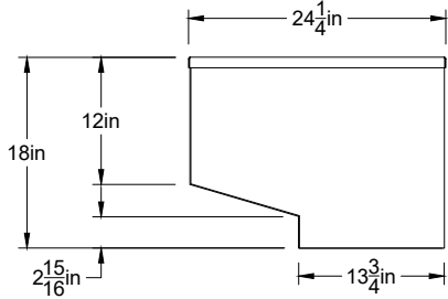
Right View Inlet Adapter Scale = 1:20
