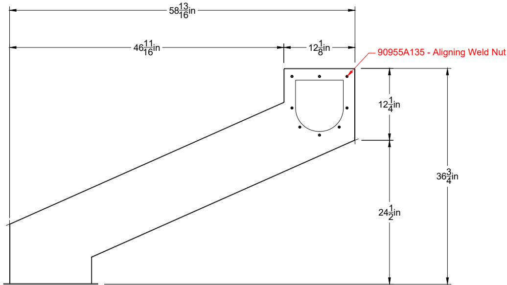
Front View Duct Unit1 Scale = 1:16
