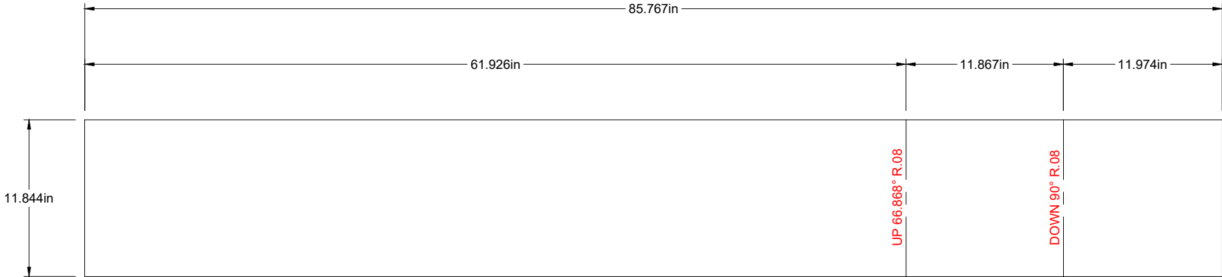
Top View U2AT (x1) 14 ga Stainless Scale = 1:10
