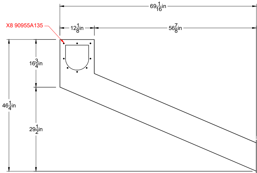
Front View Duct Unit 2-A Scale = 1:20
