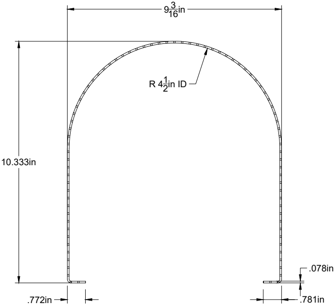
Front View Perf. Wrap Scrap (x1) Alum Scale = 1:4
