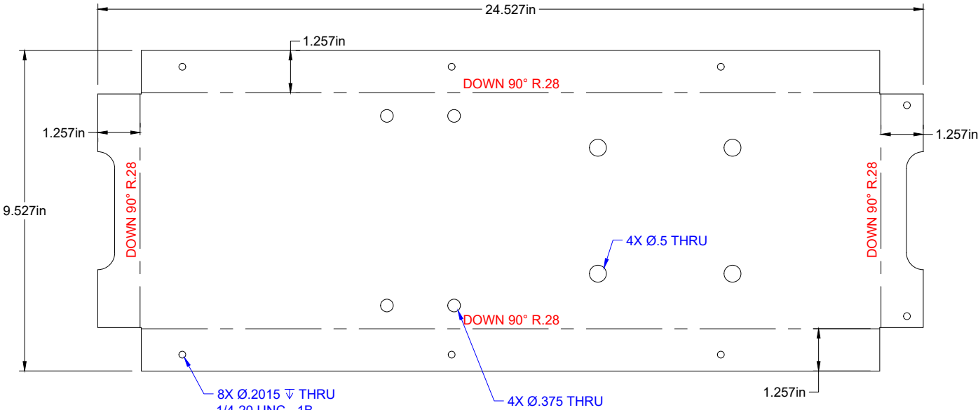
Flat Pattern Base (x1) .25 Alum Scale = 1:4
