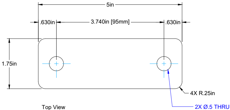
Top View SHIM(Make x2) Scale = 1:4
