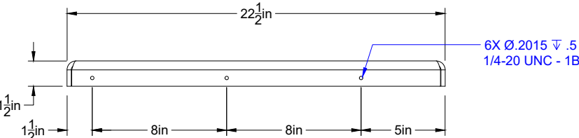
Front View Base (x1) .25 Alum Scale = 1:8
