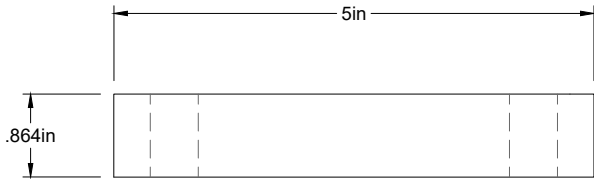
Front View SHIM(Make x2) Scale = 1:4
