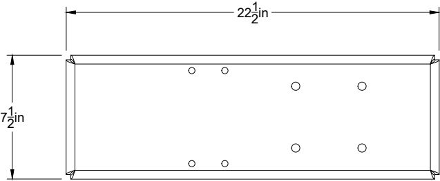
Top View Base (x1) .25 Alum Scale = 1:8
