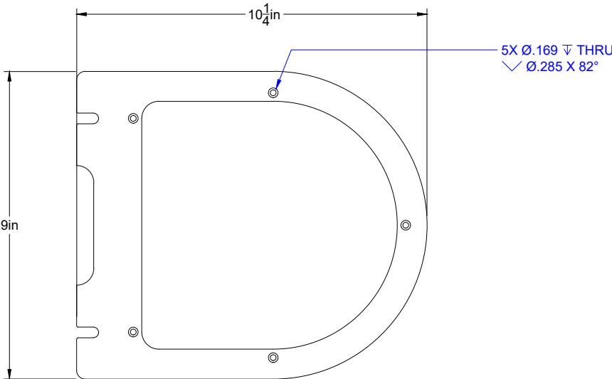
Front View BEN (x1) .125 Alum Scale = 1:4
