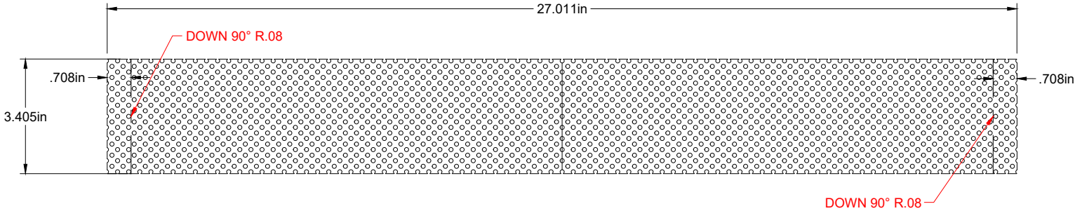
Flat Pattern Perf. Wrap Scrap (x1) Alum Scale = 1:4
