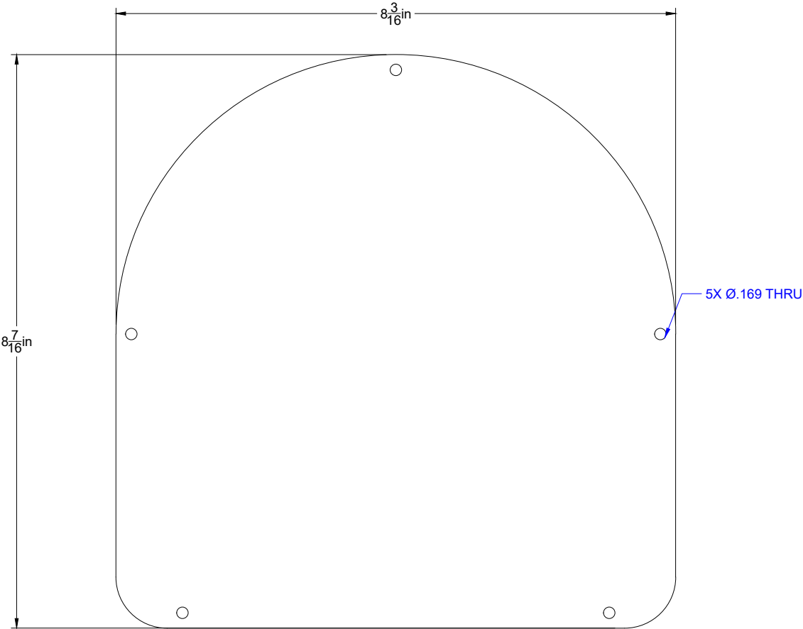
Top View Scrap Acrylic (x1) .125 Scale = 1:2
