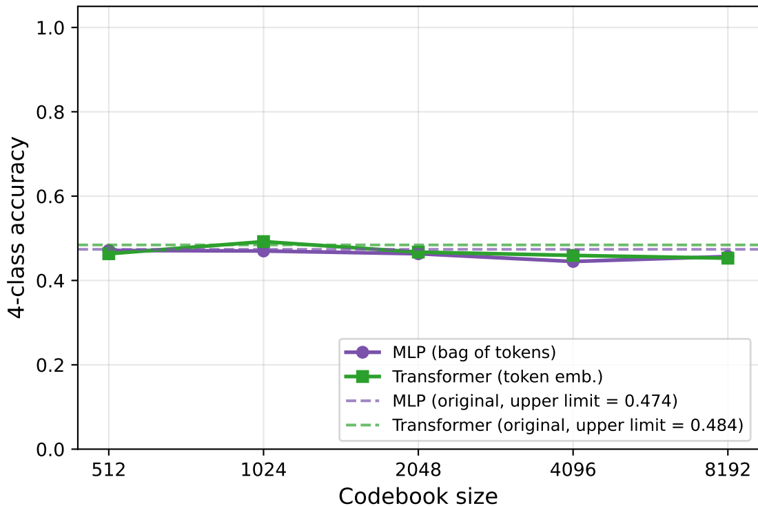
Token quality: classifier accuracy vs codebook size (L1T: minbias / QCD / ggHbb / VBFHbb)
