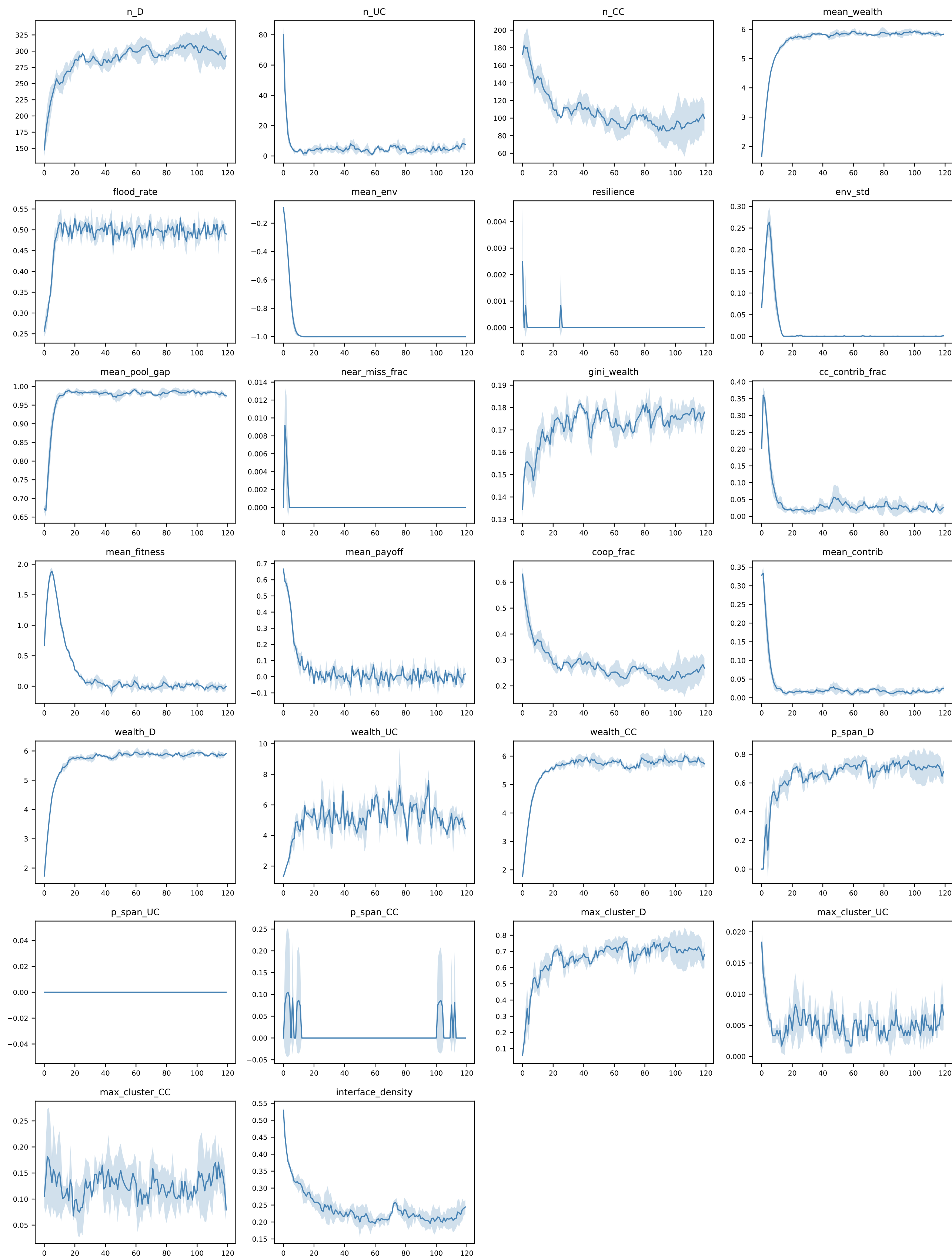
Order parameters over time (mean \pm \sigma , 3 seeds)
