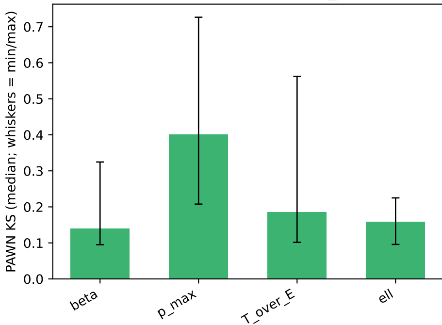
PAWN sensitivity — mean_env
