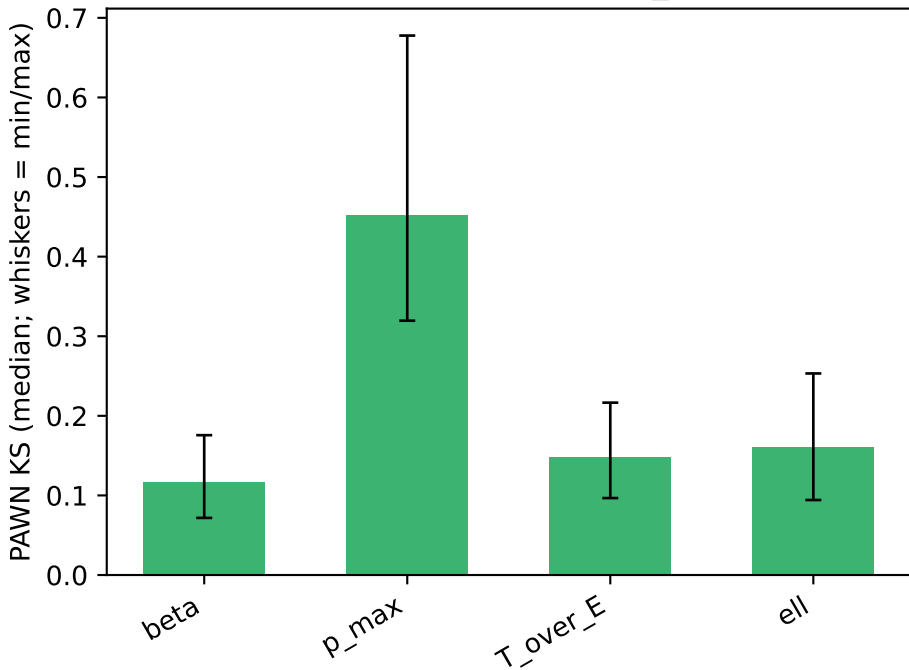
PAWN sensitivity — mean_fitness
