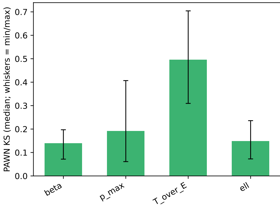
PAWN sensitivity — resilience
