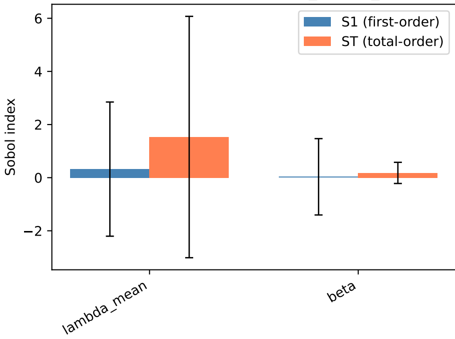
SOBOL sensitivity — max_cluster_CC
