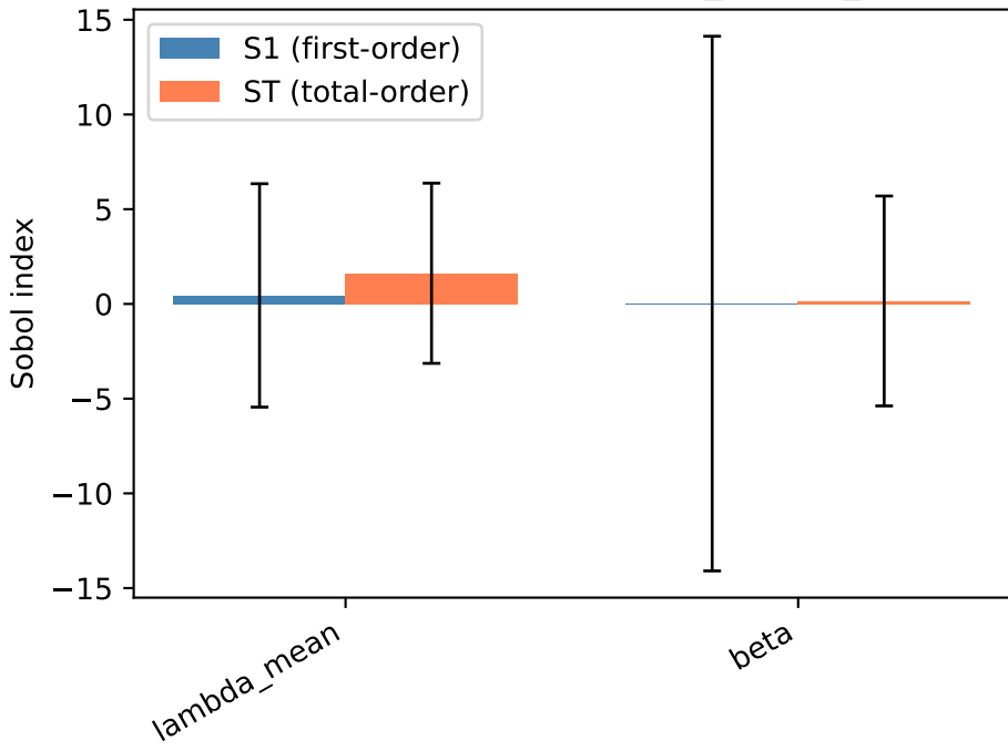
SOBOL sensitivity — max_cluster_D
