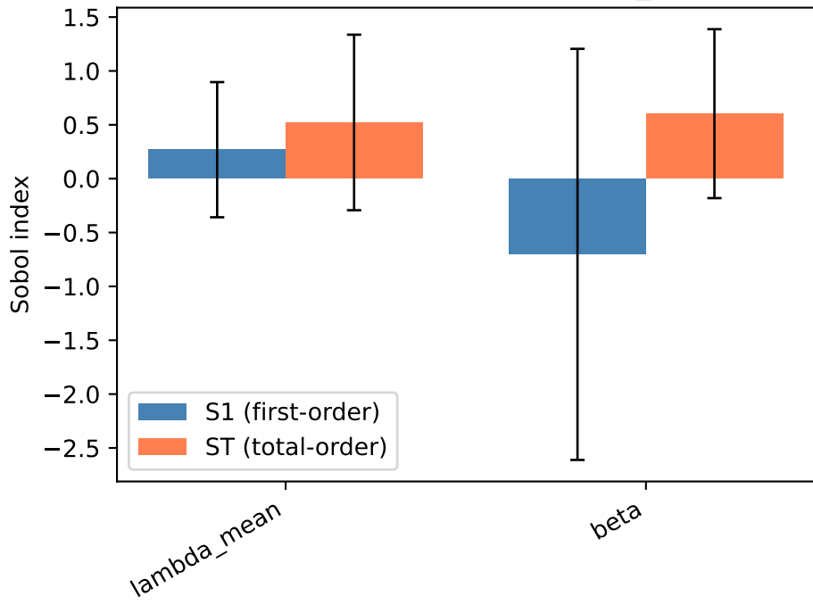
SOBOL sensitivity — wealth_CC
