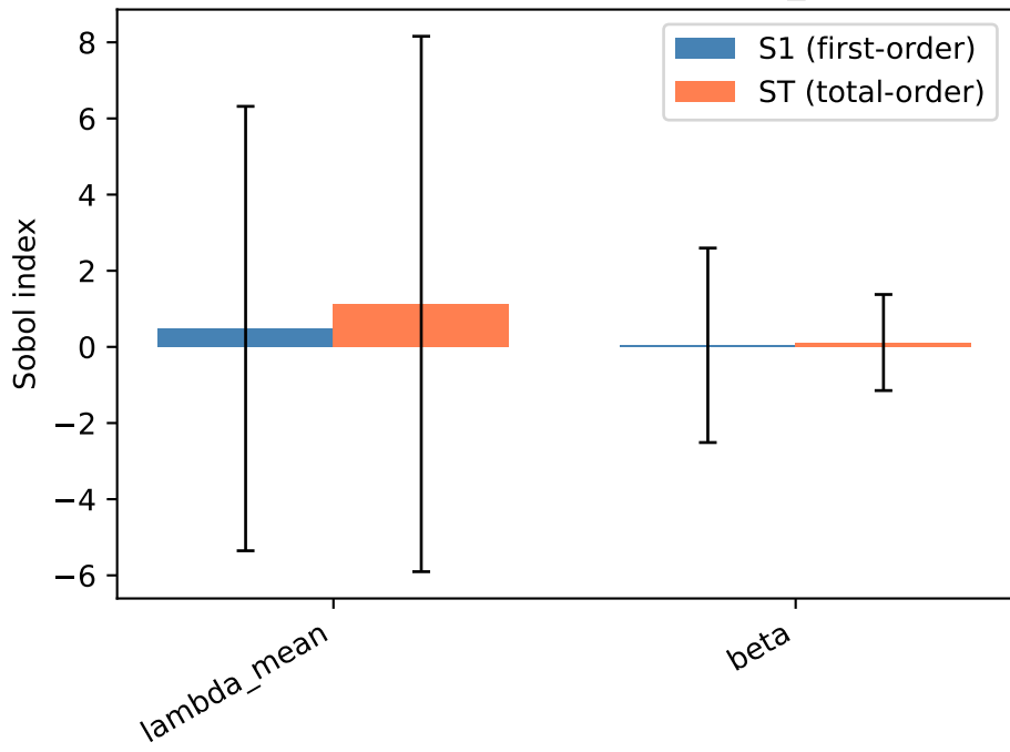
SOBOL sensitivity — wealth_D
