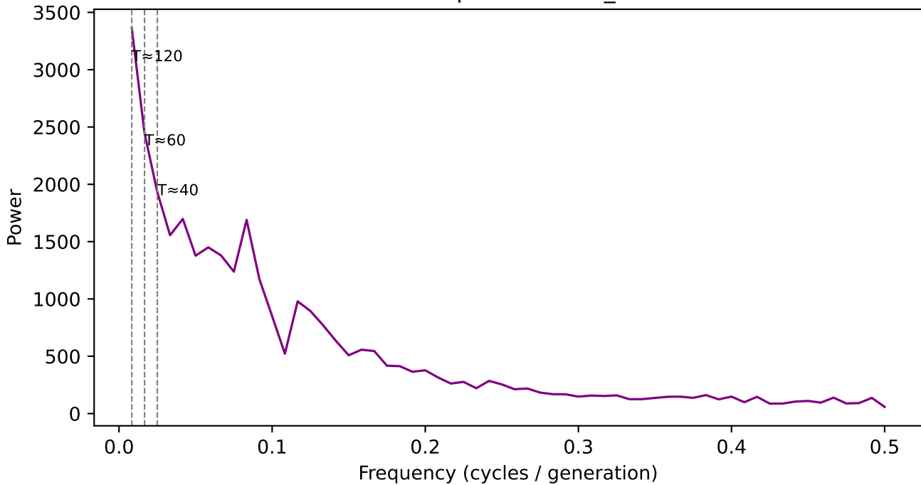
Power spectrum — n_UC
