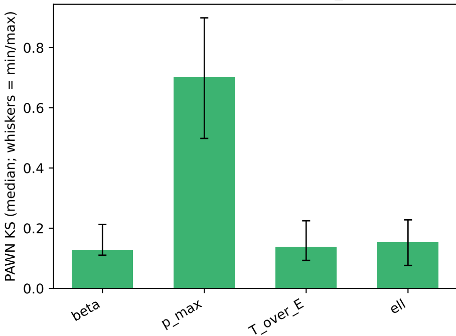
PAWN sensitivity — flood_rate
