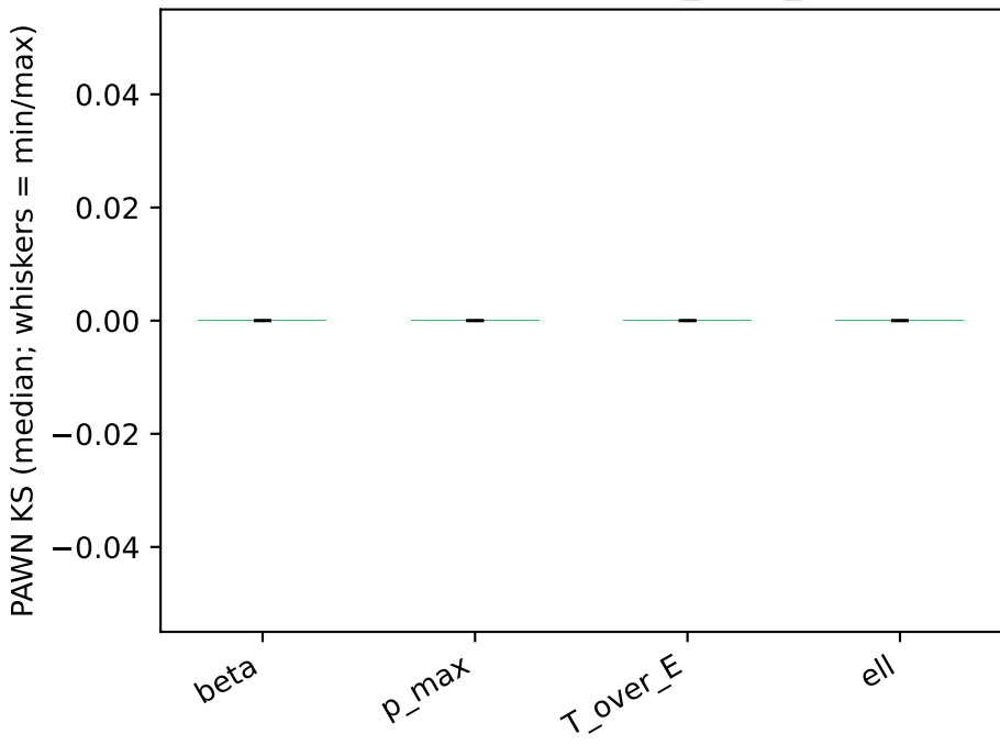
PAWN sensitivity — p_span_UC
