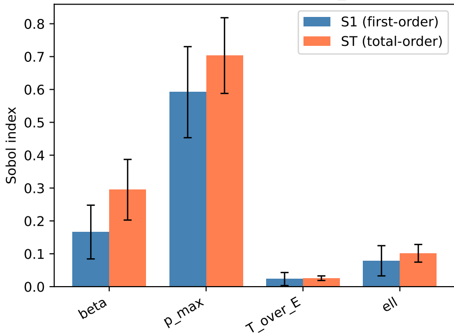
SOBOL sensitivity — coop_frac
