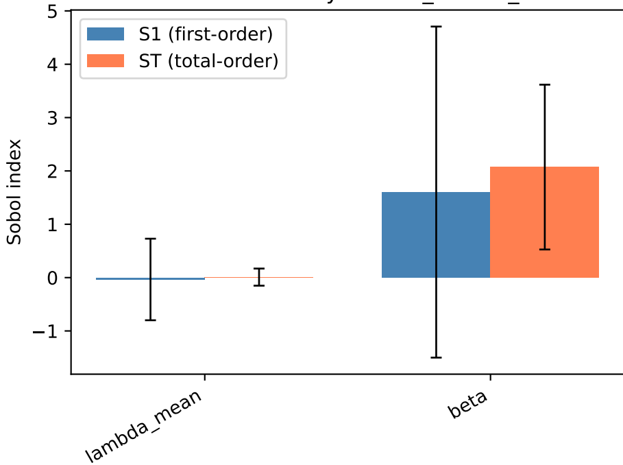
SOBOL sensitivity — max_cluster_UC
