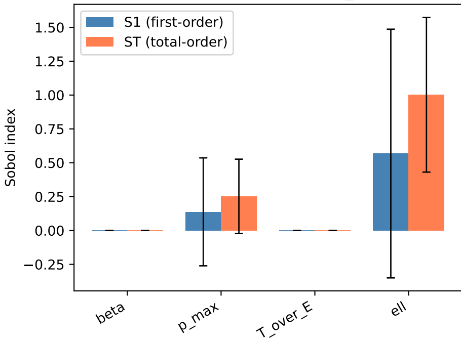
SOBOL sensitivity — mean_fitness
