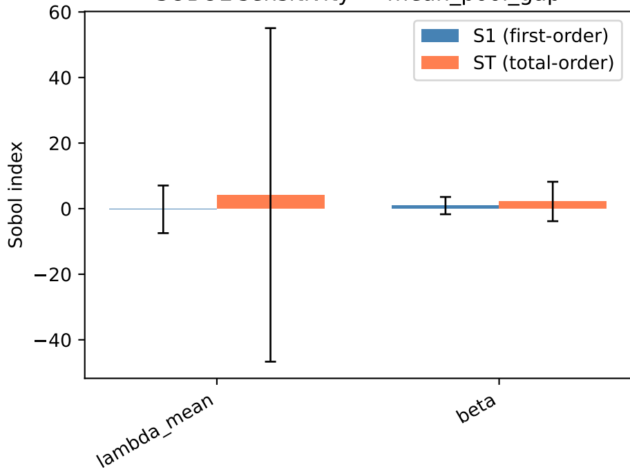
SOBOL sensitivity — mean_pool_gap
